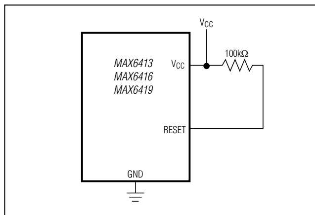
Figure 7. Ensuring \overline{\text{RESET}} Valid to VCC = 0V
