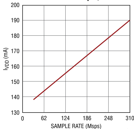
LTC2153-14: I_{VDD} vs Sample Rate, 15MHz Sine Wave Input, -1dBFS
