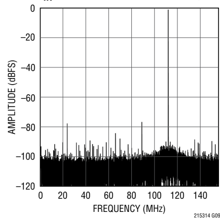
LTC2153-14: 32K Point FFT, f_{IN} = 421\text{MHz} , -1\text{dBFS} , 310Msps
