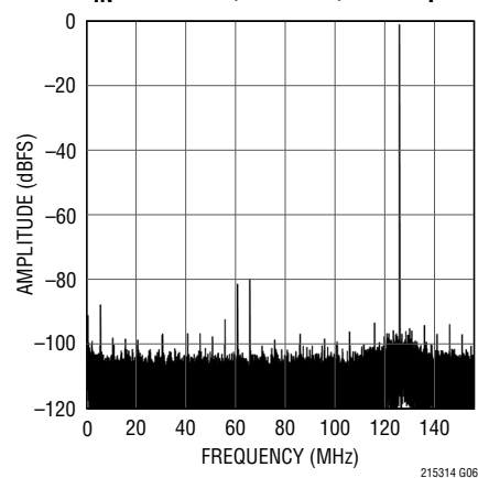
LTC2153-14: 32K Point FFT, f_{IN} = 185\text{MHz} , -1\text{dBFS} , 310Msps
