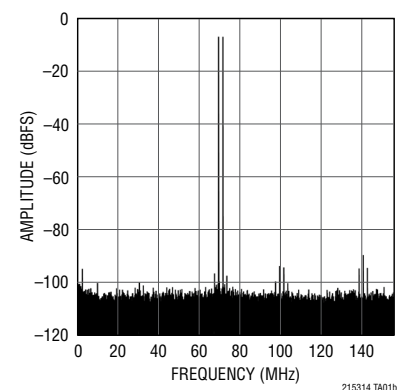
LTC2153-14 32K Point 2-Tone FFT, f IN = 71MHz and 69MHz, 310Msps
