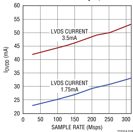
LTC2153-14: I_{OVD} vs Sample Rate, 15MHz Sine Wave Input, -1dBFS
