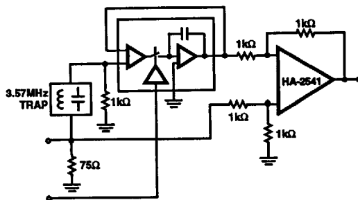
FIGURE 18. VIDEO DC RESTORER
