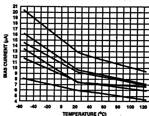
FIGURE 5. BIAS CURRENT DRIFT WITH TEMPERATURE (6 REPRESENTATIVE UNITS)
