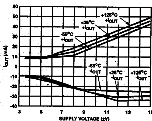
FIGURE 7. OUTPUT CURRENT vs SUPPLY VOLTAGE (AT VARIOUS TEMPERATURES)
