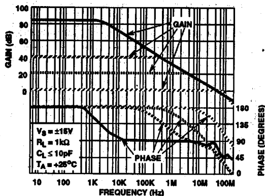
FIGURE 14. GAIN AND PHASE FREQUENCY RESPONSE
