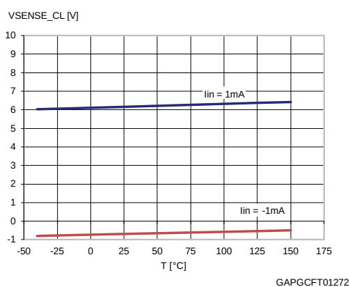
Figure 33: V_{sense\_CL} vs. T_{case}
