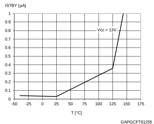
Figure 16: Standby current
