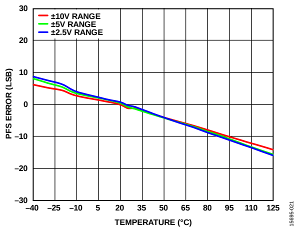
Figure 21. PFS Error vs. Temperature
