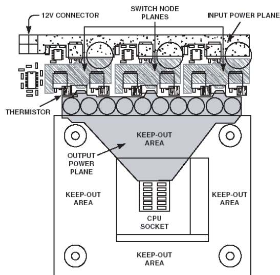
Figure 11. Layout Recommendations
