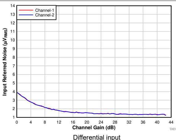
Figure 7-13. Input-Referred Noise vs Channel Gain
