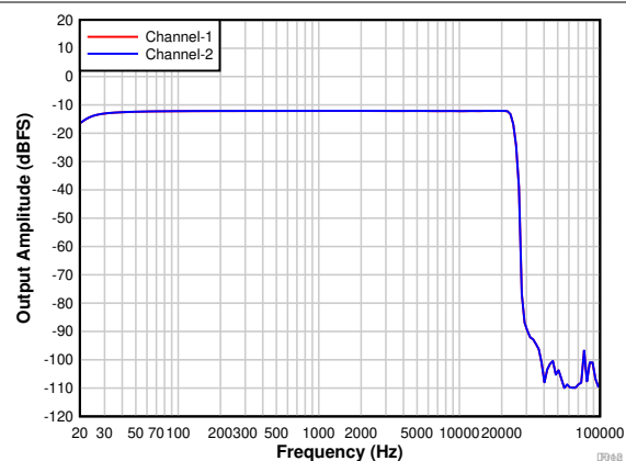
Figure 7-15. Frequency Response With a -12\text{-dBr} Input
