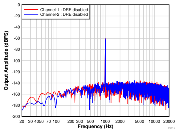
Figure 7-20. Differential FFT With a -60-dBr Input With DRE Disabled
