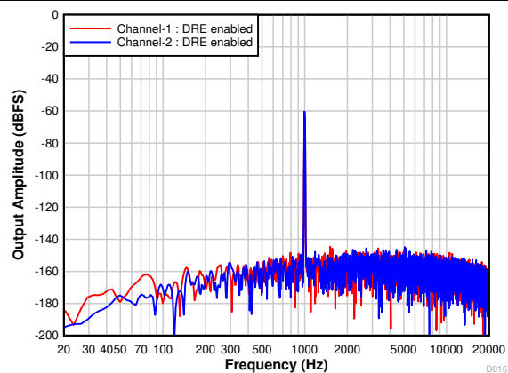
Figure 7-19. Differential FFT With a -60-dBr Input With DRE Enabled
