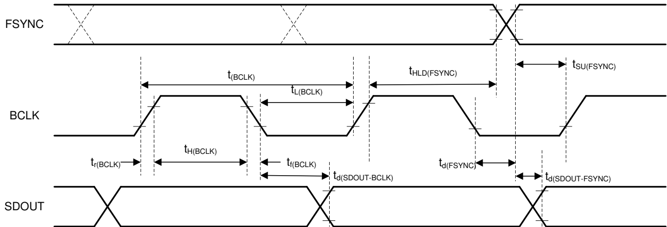
Figure 7-2. TDM (With BCLK_POL = 1), I²S, and LJ Interface Timing Diagram
