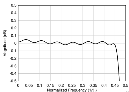
Figure 8-20. Linear Phase Decimation Filter Pass-Band Ripple
