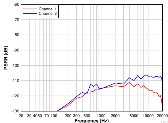
Figure 7-16. Power-Supply Rejection Ratio vs Ripple Frequency With 100-mV PP Amplitude
