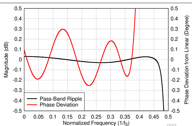
Figure 8-48. Low-Latency Decimation Filter Pass-Band Ripple and Phase Deviation
