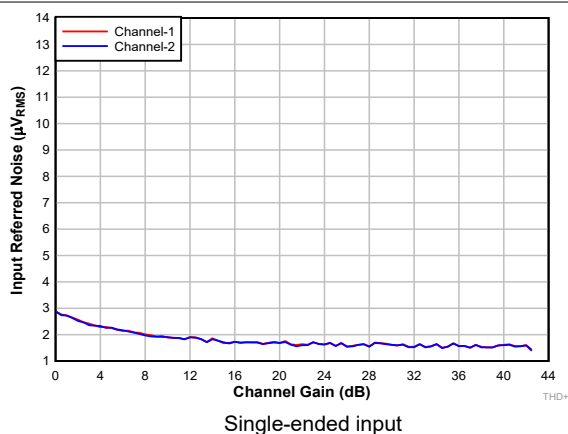
Figure 7-14. Input-Referred Noise vs Channel Gain
