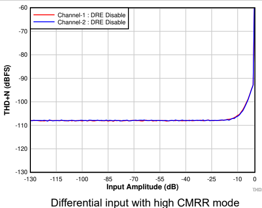
Figure 7-30. THD+N vs Input Amplitude With DRE Disabled
