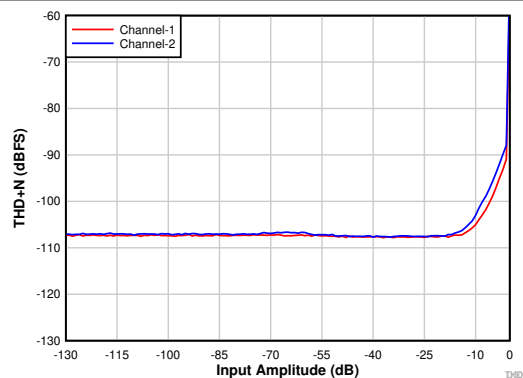
Figure 7-9. THD+N vs Input Amplitude With DRE Disabled
