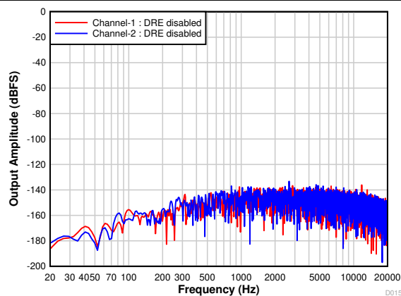
Figure 7-18. Differential FFT With Idle Input With DRE Disabled
