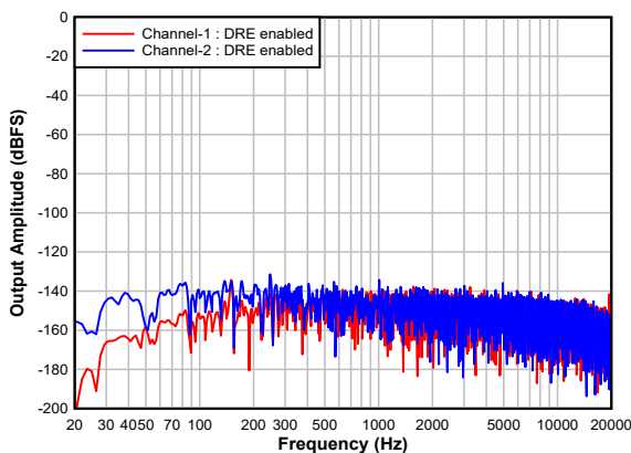
Figure 7-21. Single Ended FFT With Idle Input With DRE Enabled
