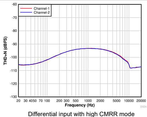
Figure 7-31. THD+N vs Input Frequency at -1-dBr Input With DRE Disabled
