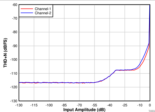
Figure 7-8. THD+N vs Input Amplitude With DRE Enabled
