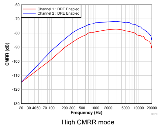
Figure 7-27. Common-Mode Rejection Ratio vs Ripple Frequency With 100-mV PP Amplitude and DRE Enabled
