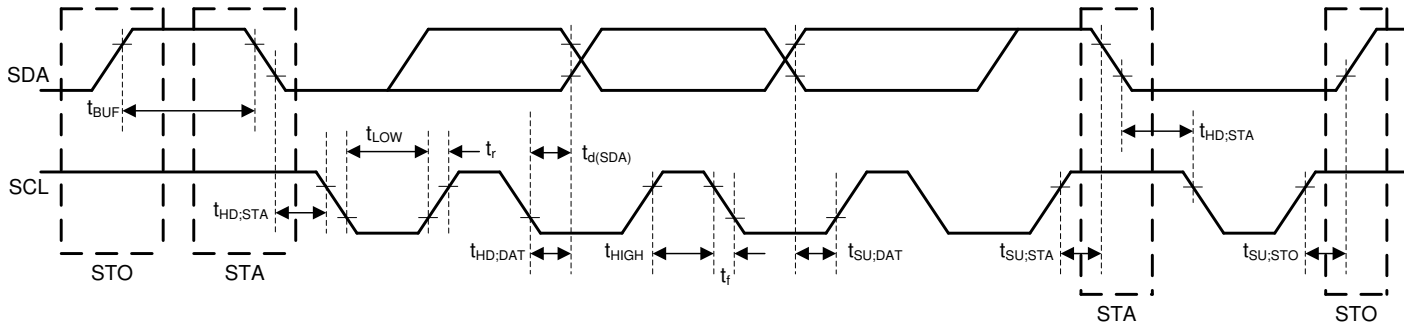
Figure 7-1. I²C Interface Timing Diagram
