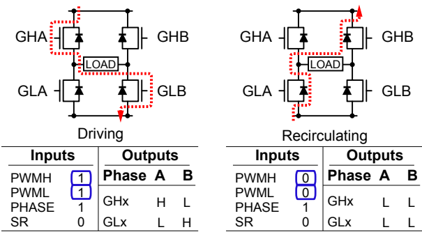
(A) Fast Decay, Diode Rectification
