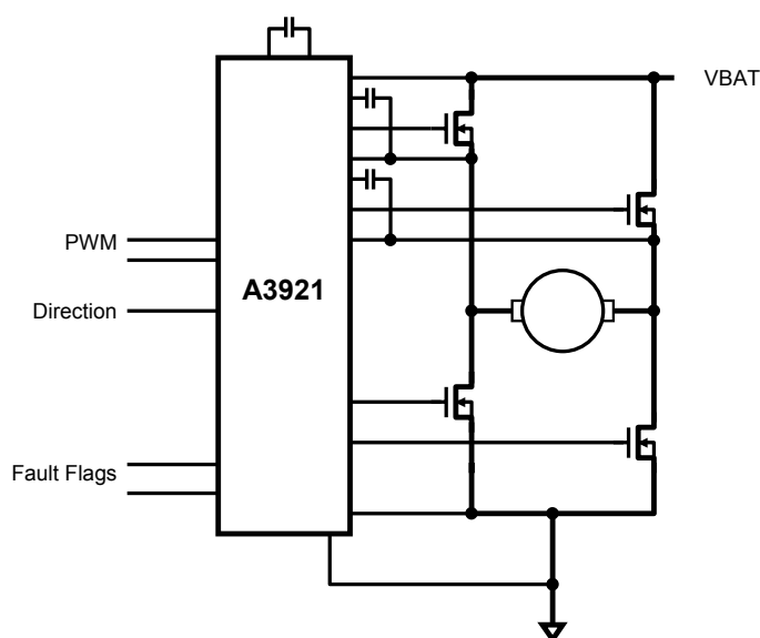
Typical Application
