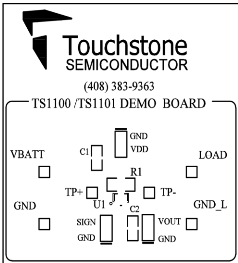
Figure 2. Top Layer Component View
