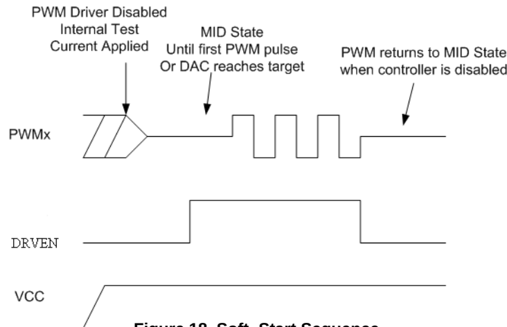
Figure 18. Soft-Start Sequence
