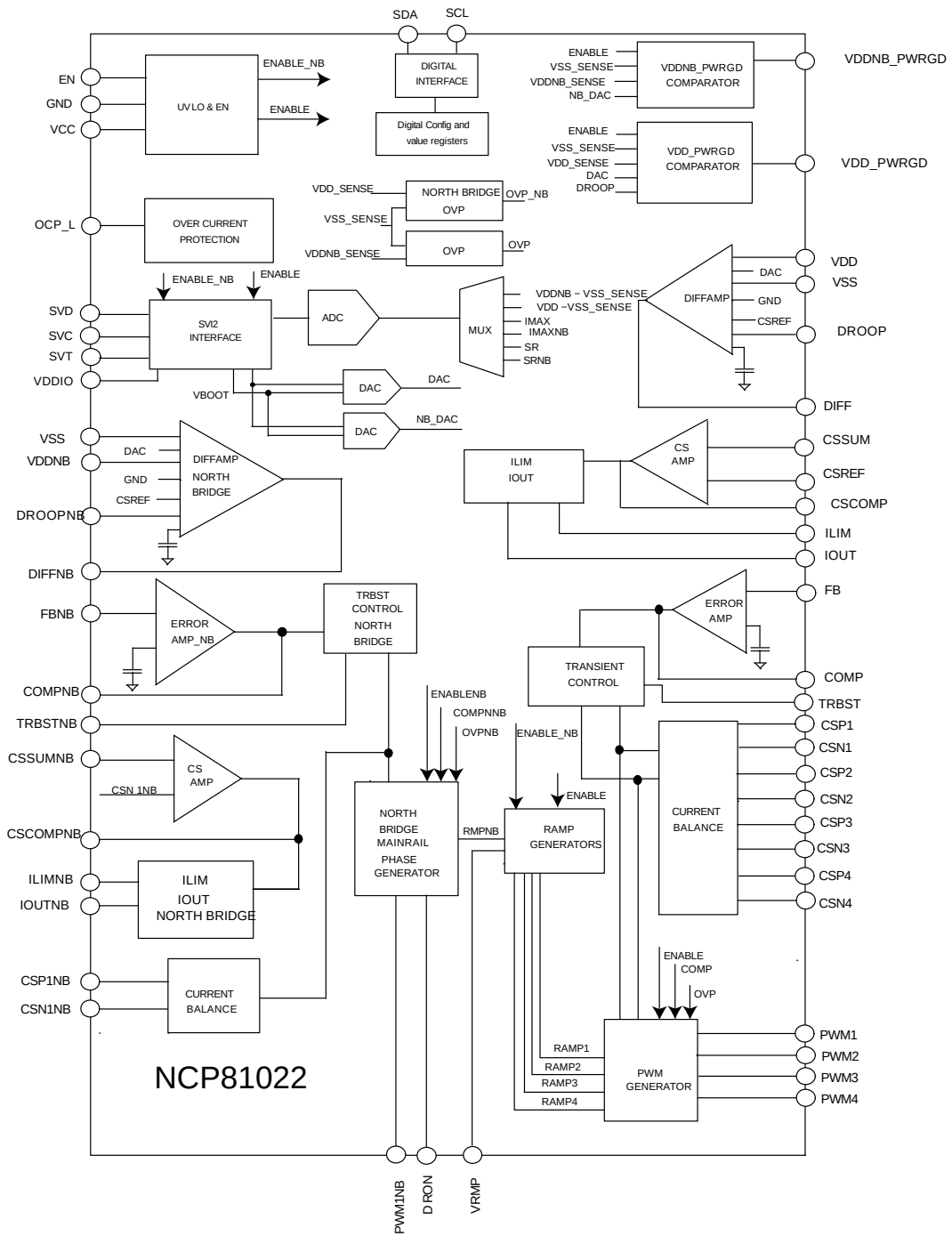
Figure 1. Block Diagram
