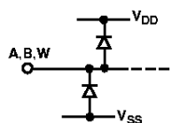
Figure 44. Equivalent ESD Protection Analog Pins
