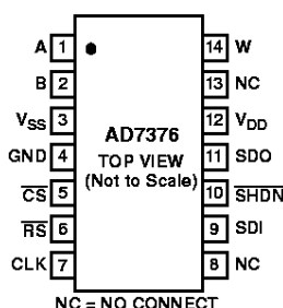
PDIP &amp; TSSOP-14
