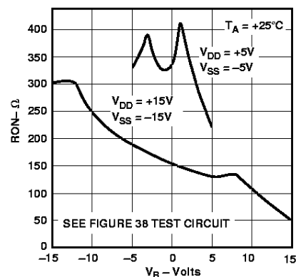
Figure 25. Incremental Wiper Contact Resistance vs. Common-Mode Voltage
