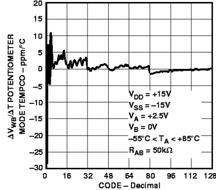
Figure 9. ΔV WB /ΔT Potentiometer Mode Tempco
