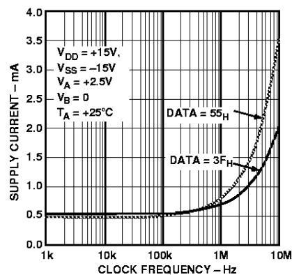
Figure 28. I_{DD} Supply Current vs. Input Clock Frequency
