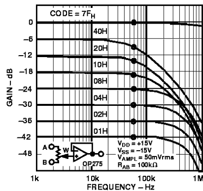
Figure 20. 100 kΩ Gain vs. Frequency vs. Code
