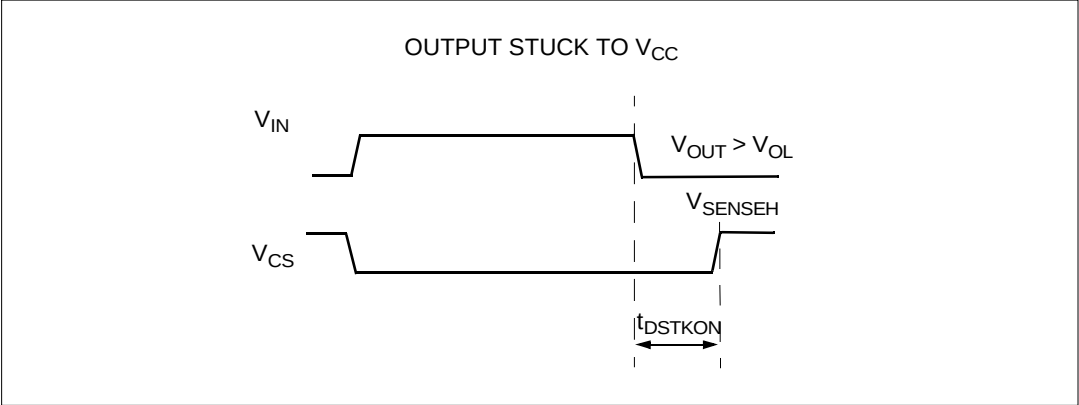
Figure 6. Switching characteristics
