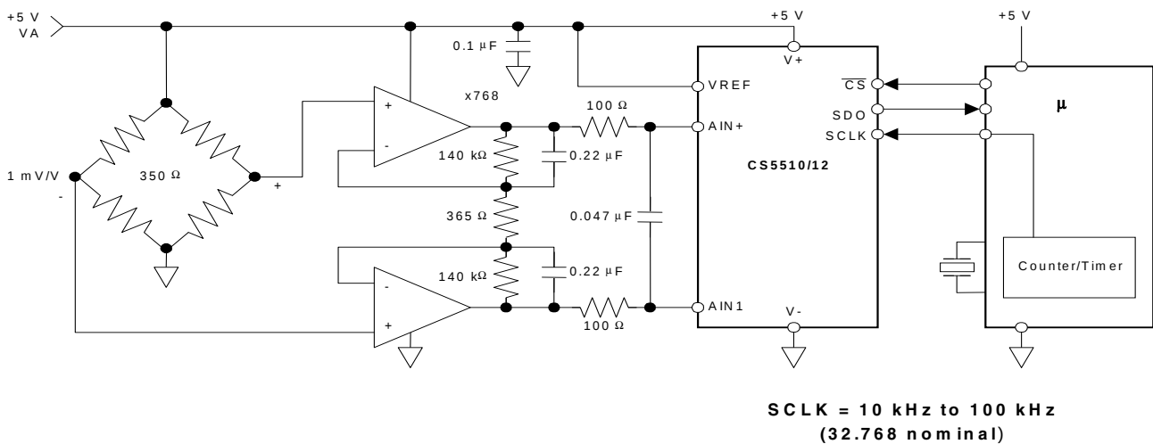
Figure 20. Load Cell Bridge Amplifier and A/D Converter
