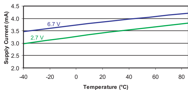
Figure 6. Supply Current vs. Temperature, CS3002
