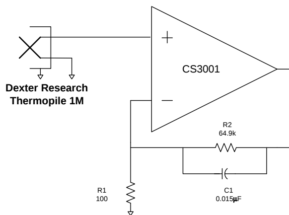
Thermopile Amplifier with a Gain of 650 V/V
