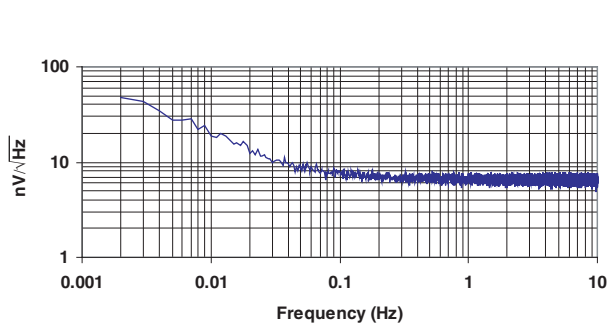
Figure 1. Noise vs. Frequency (Measured)
