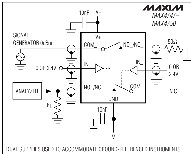
Figure 6. Crosstalk
