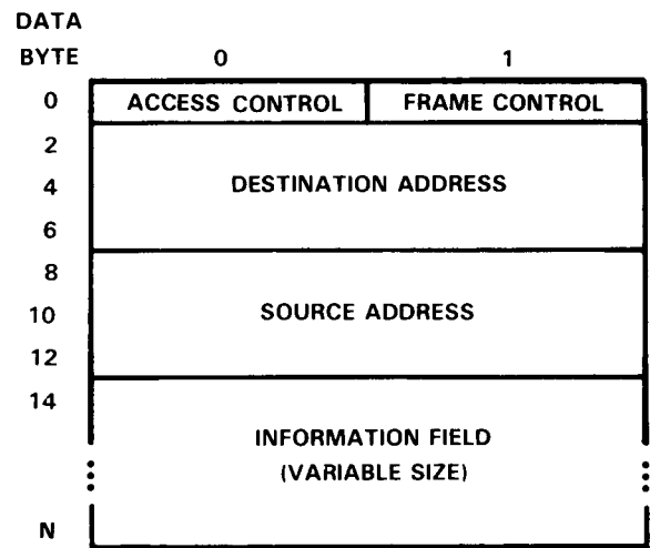
FIGURE 5. TRANSMIT DATA FORMAT
