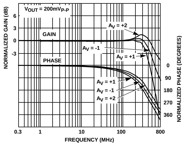
FIGURE 12. FREQUENCY RESPONSE
