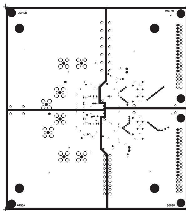
Figure 6d. Layer 2
