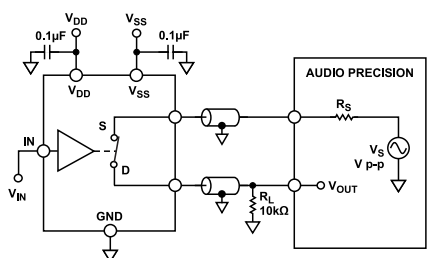
Figure 37. THD + Noise
