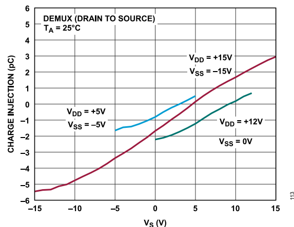
Figure 14. Charge Injection vs. V_S , Drain-to-Source
