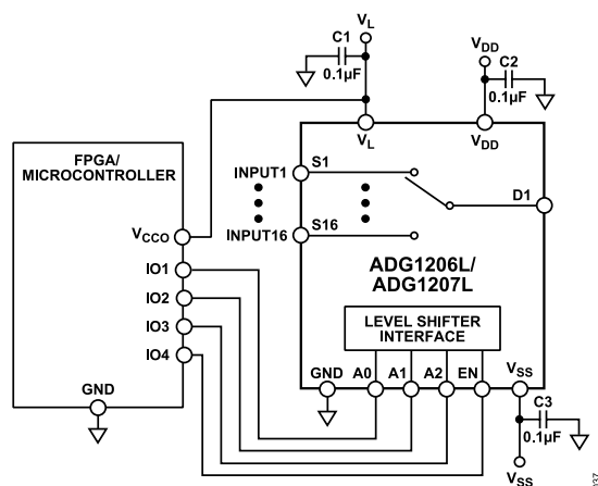
Figure 38. Typical Application
