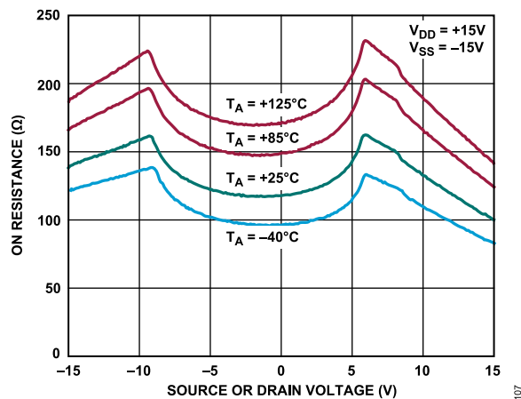
Figure 8. On Resistance as a Function of V_D ( V_S ) for Different Temperatures, Dual Supply
