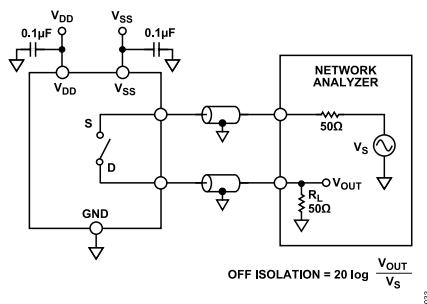
Figure 34. Off Isolation
