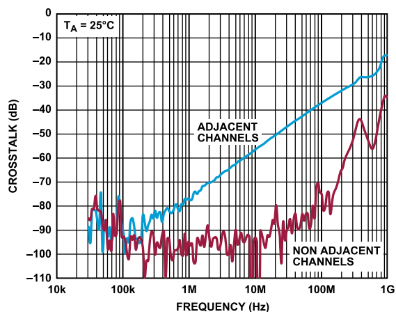
Figure 18. Crosstalk vs. Frequency, ADG1207L
