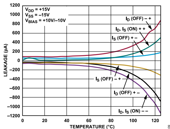
Figure 10. ADG1206L Leakage Currents as a Function of Temperature, Dual Supply
