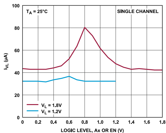
Figure 12. I_{OL} vs. Logic Level
