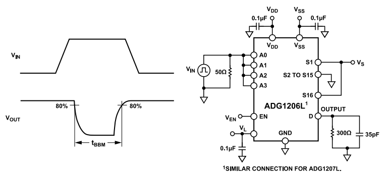
Figure 31. Break-Before-Make Delay, t_{\text{BBM}}
