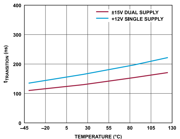
Figure 15. Transition Time ( t_{\text{TRANSITION}} ) vs. Temperature
