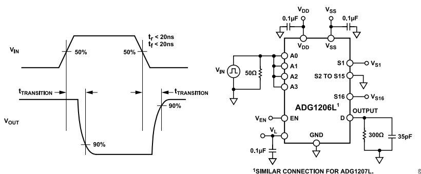
Figure 30. Address to Output Switching Times, t_{\text{TRANSITION}} ( V_{\text{OUT}} is the Output Voltage)
