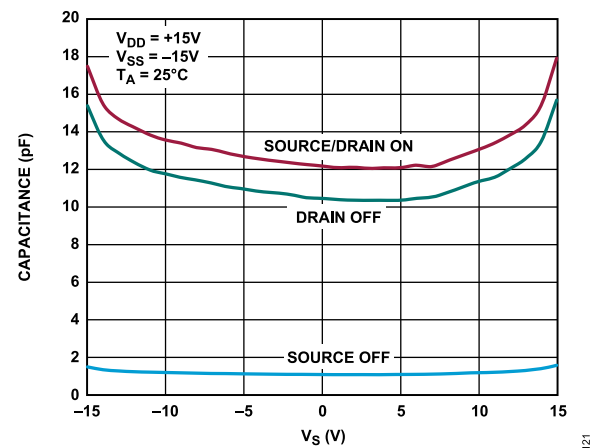
Figure 22. Capacitance vs. V_S , \pm 15 V Dual Supply, ADG1206L
