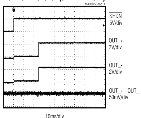
TURN-ON RESPONSE (SPEAKER MODE)
