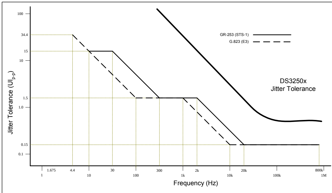
Figure 9-4. STS-1 and E3 Jitter Tolerance
