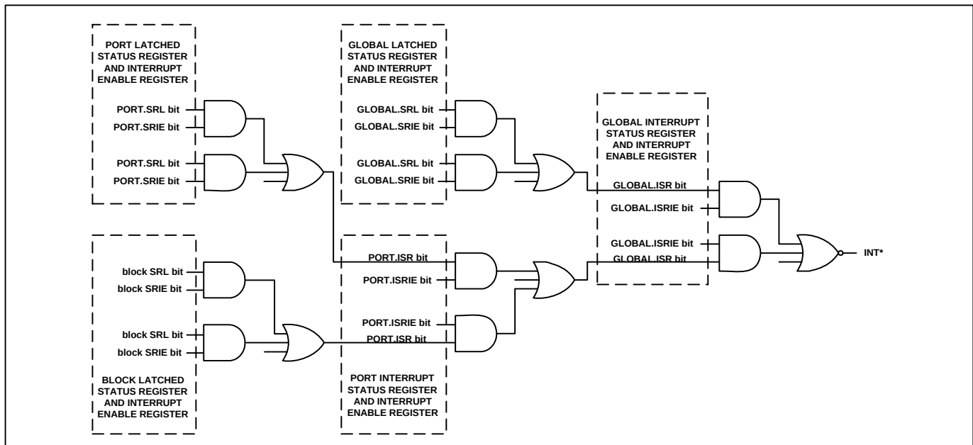
Figure 9-12. Interrupt Signal Flow
