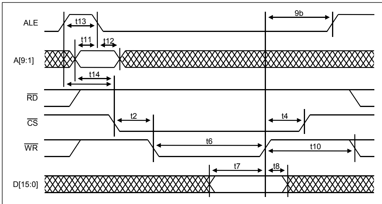
Figure 12-8. Parallel CPU Interface Intel Write Timing Diagram (Multiplexed)
