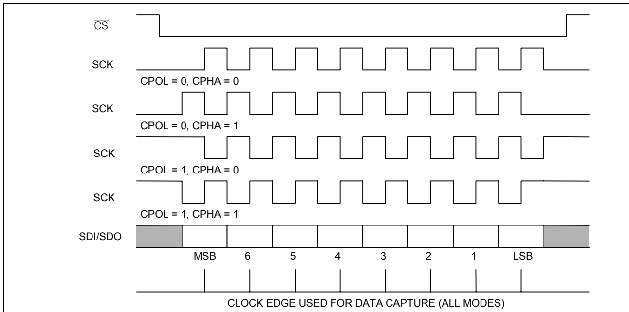
Figure 9-11. SPI Bus Transactions
