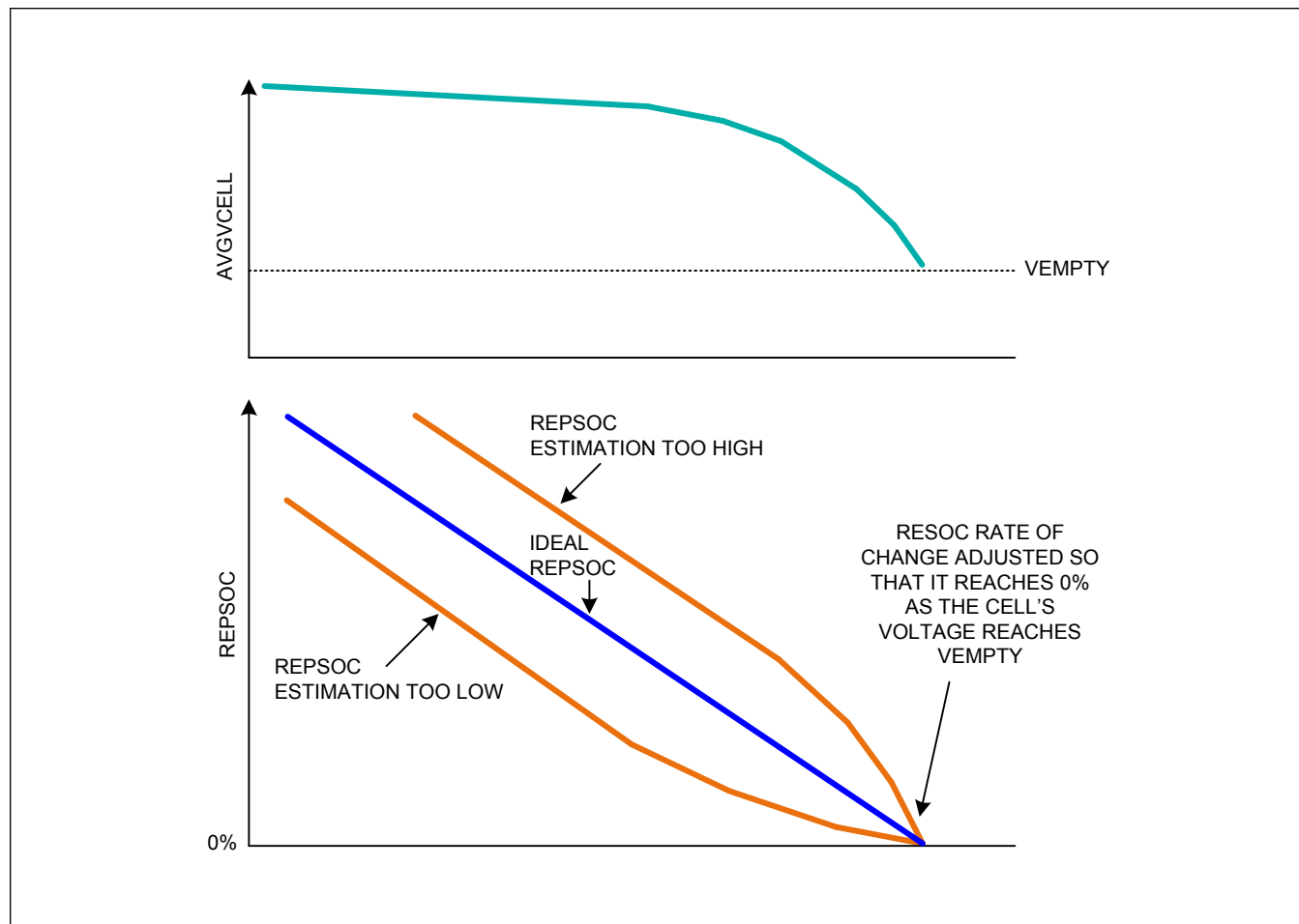
Figure 21. Converge-To-Empty
