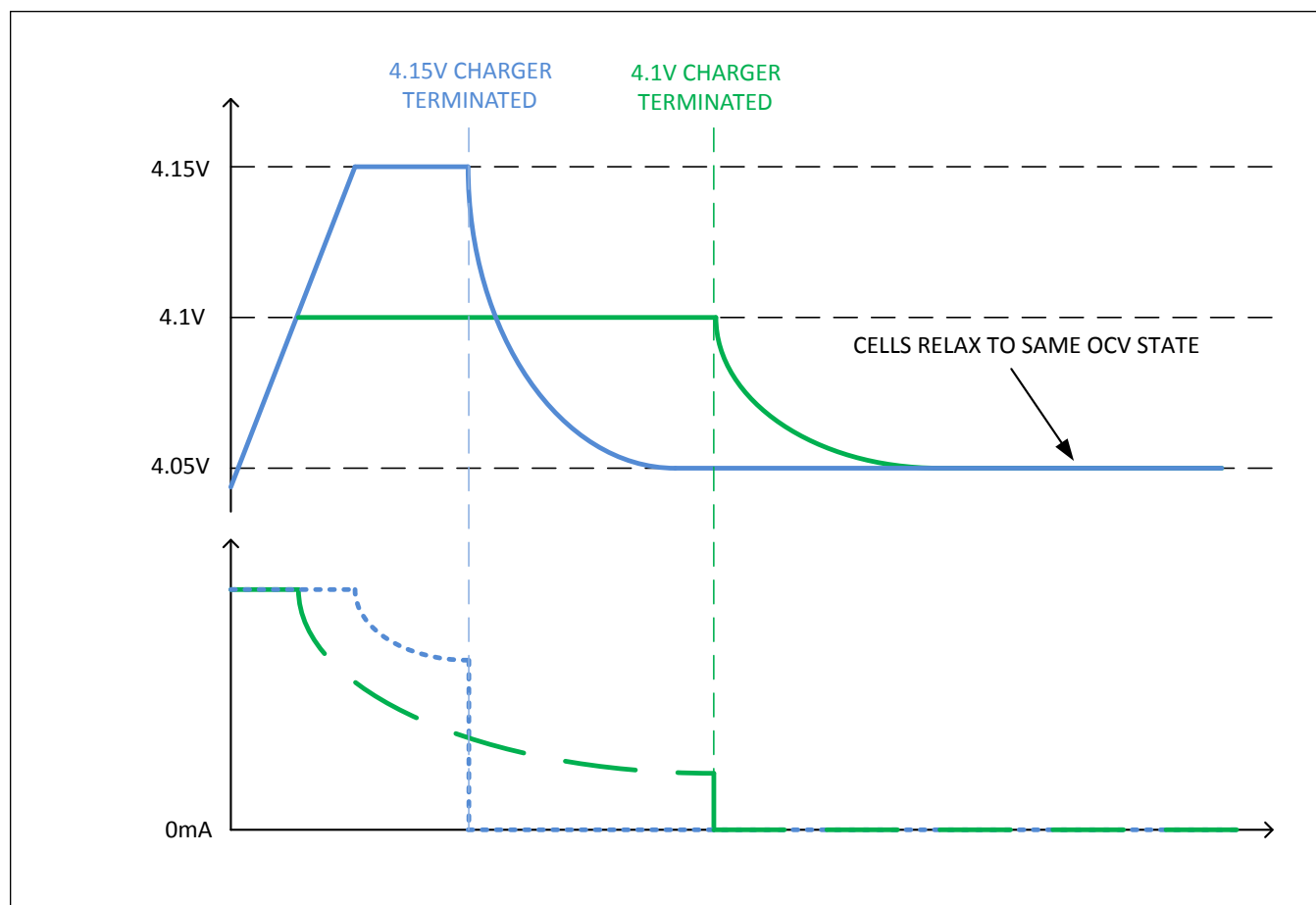
Figure 19. Smart-Full Example
