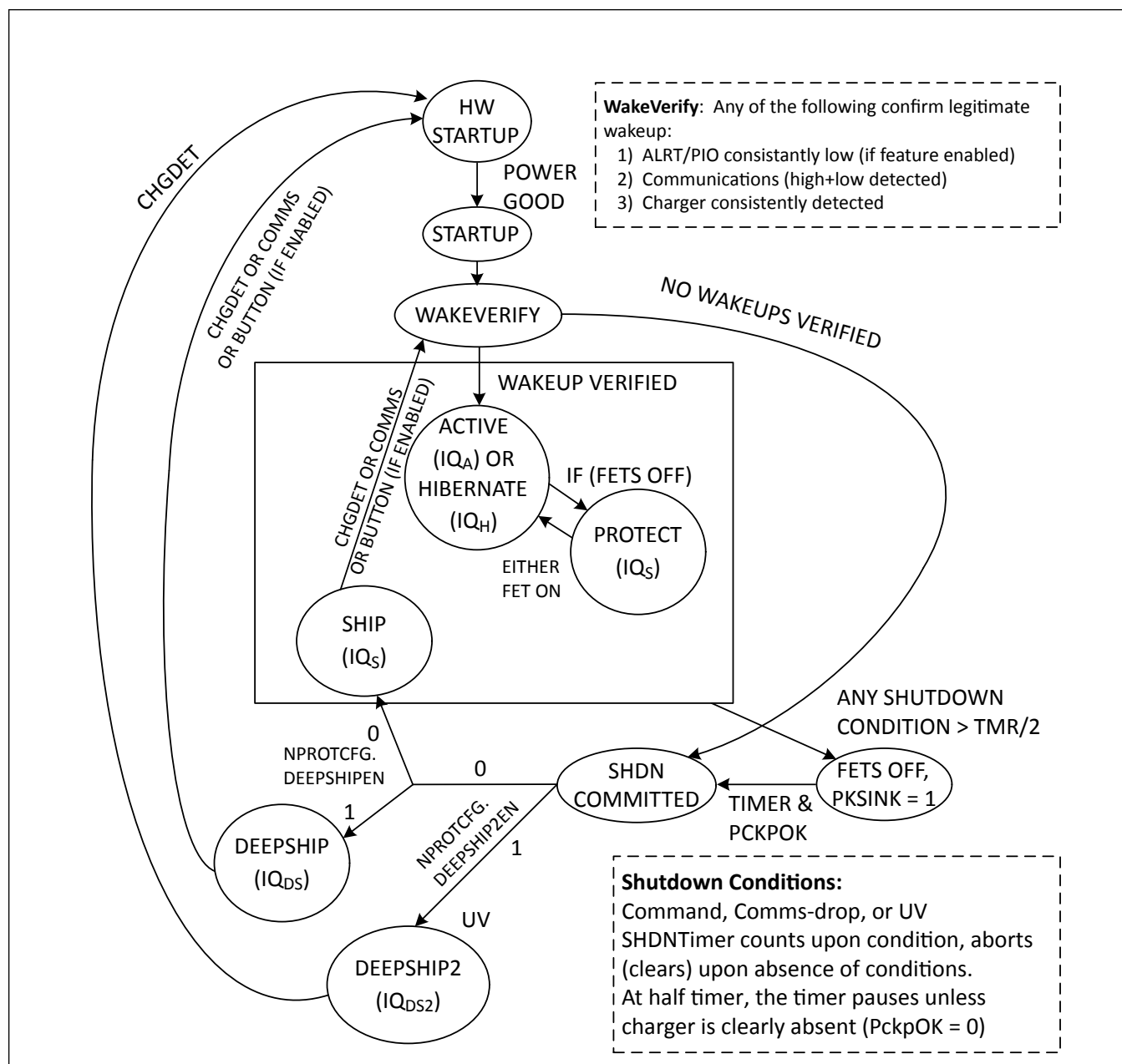
Figure 12. Power Mode Transition State Diagram
