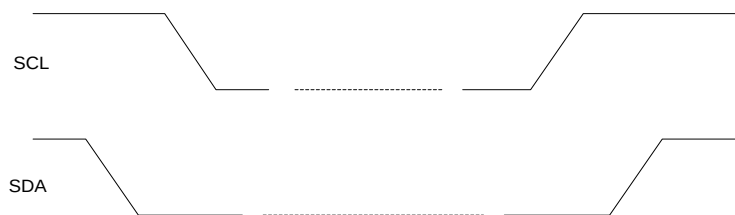
Figure 34: I 2 C START and STOP Conditions
