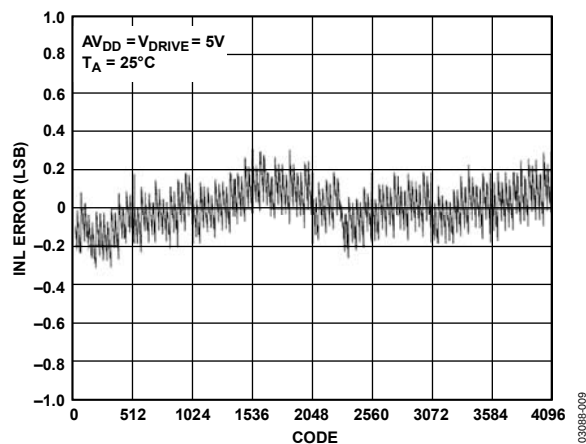
Figure 9. Typical INL
