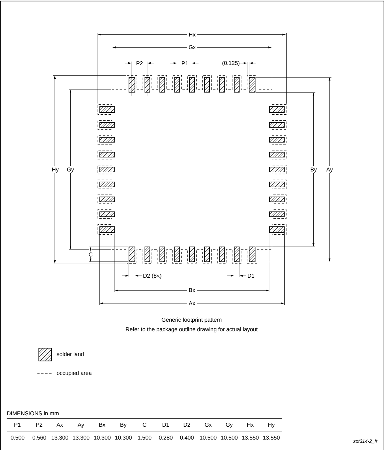
Fig 36. LQFP64 Soldering footprint
