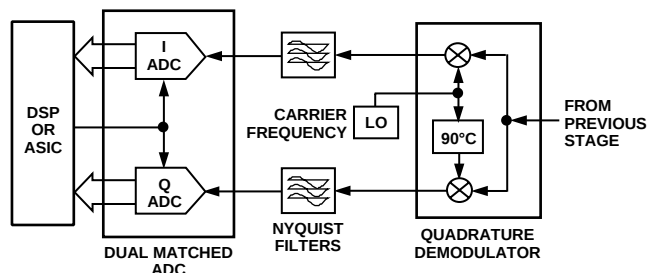
Figure 32. Typical Analog QAM Demodulator
