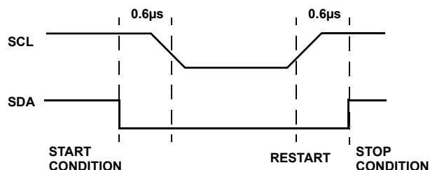
FIGURE 1. WATCHDOG RESTART
