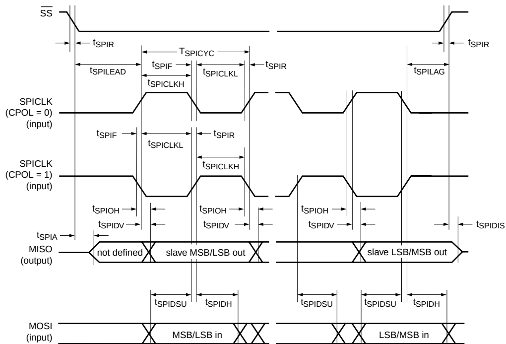
Fig 21. SPI slave timing (CPHA = 1)
