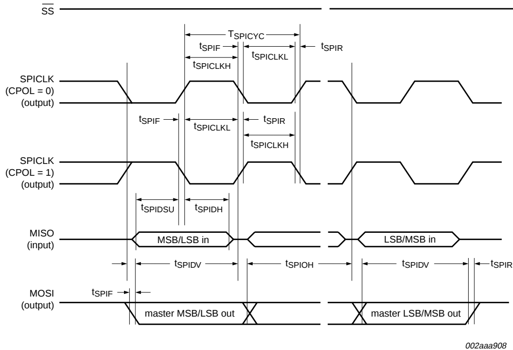
Fig 18. SPI master timing (CPHA = 0)
