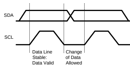
Figure 8. Bit Transfer
