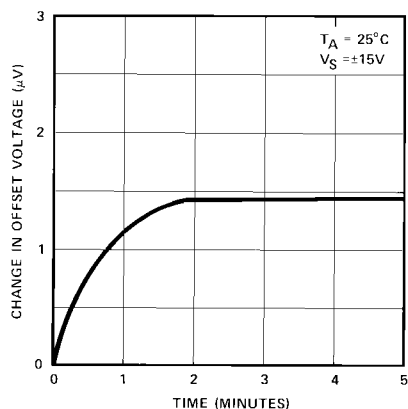
WARM-UP DRIFT
