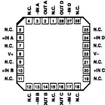
28-LEAD LCC (TC-Suffix)
