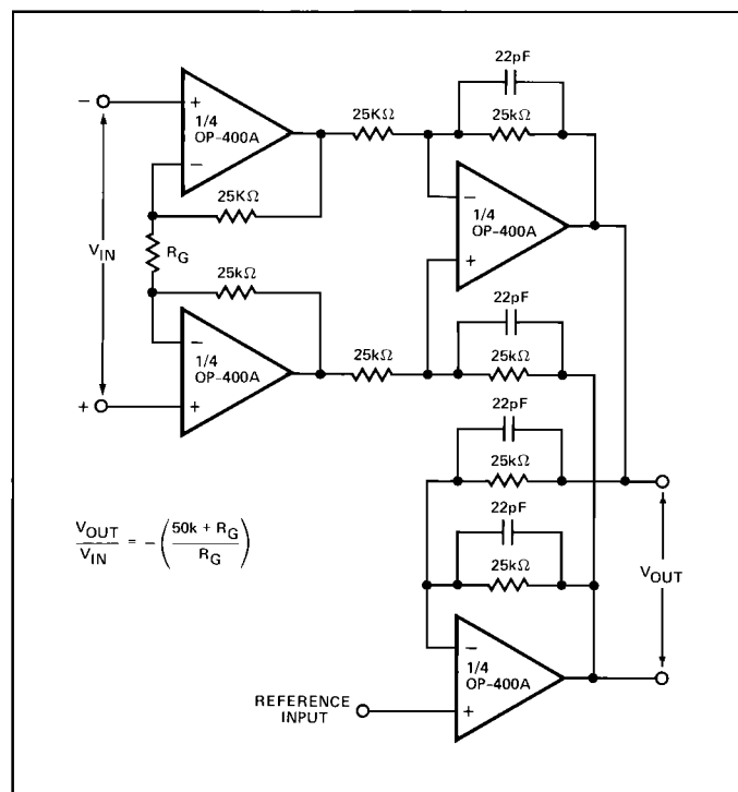
FIGURE 3: Differential Output Instrumentation Amplifier
