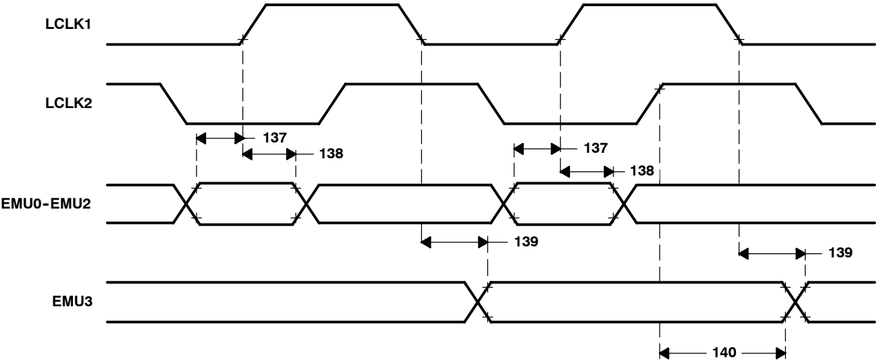
Figure 58. Emulator-Interface Timing
