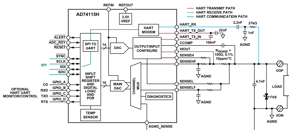
Figure 52. HART Configuration
