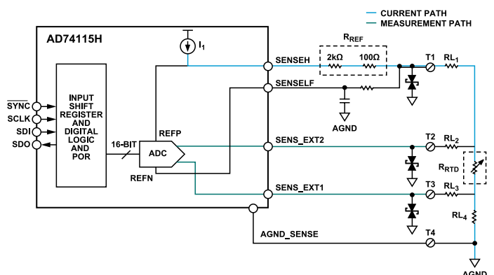
Figure 41. 4-Wire RTD Measurement Configuration
