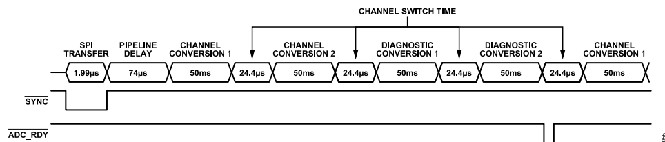
Figure 54. Multiple Measurements, Continuous Conversions Timing Diagram
