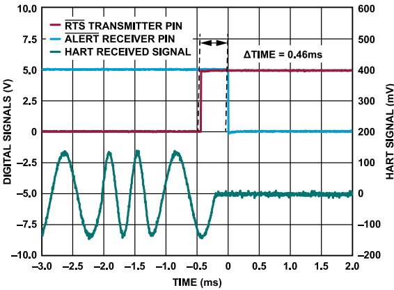
Figure 30. Carrier Detect Off Time (Till \overline{\text{ALERT}} Pin Change to High)
