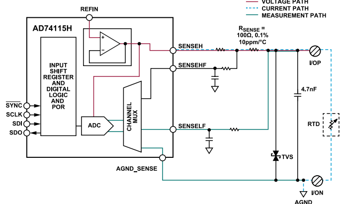
Figure 39. Resistance Measurement Configuration
