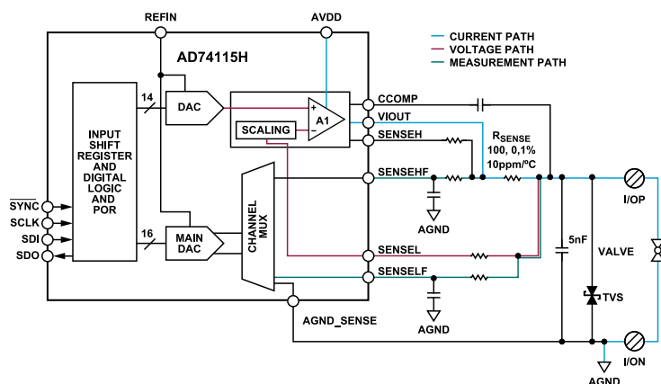
Figure 33. Voltage Output Mode Configuration
