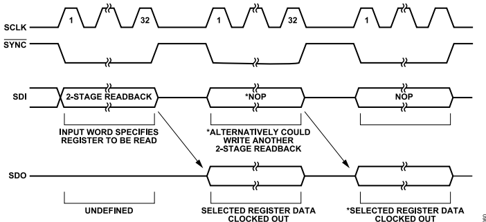
Figure 59. 2-Stage Readback Timing Diagram
