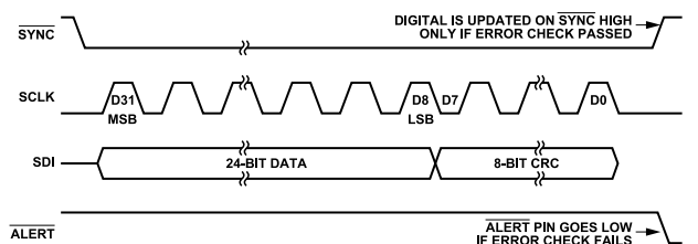
Figure 61. CRC Timing
