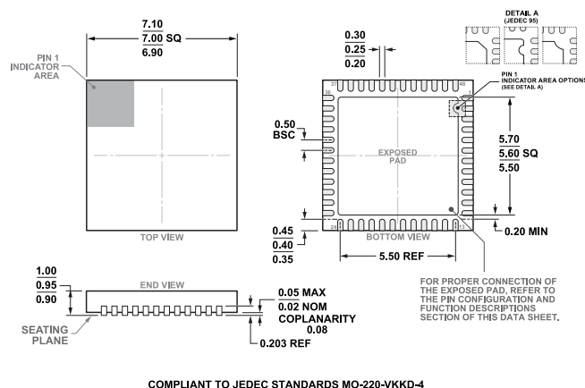
Figure 64. 48-Lead Lead Frame Chip Scale Package [LFCSP] 7 mm × 7 mm Body and 0.95 mm Package Height (CP-48-28) Dimensions shown in millimeters
