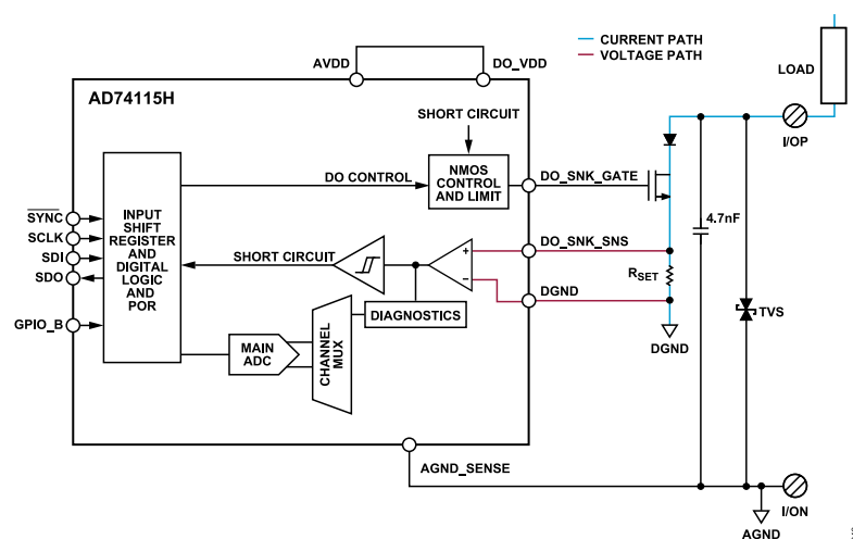
Figure 47. Digital Output Sinking with External FET
