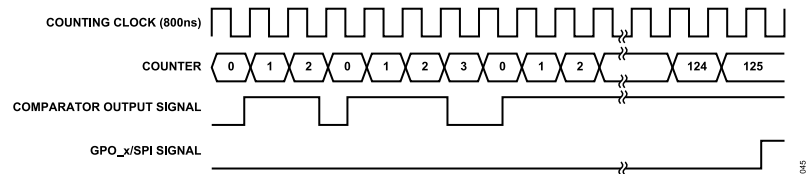
Figure 44. Digital Input Debounce Mode 1 Timing Example
