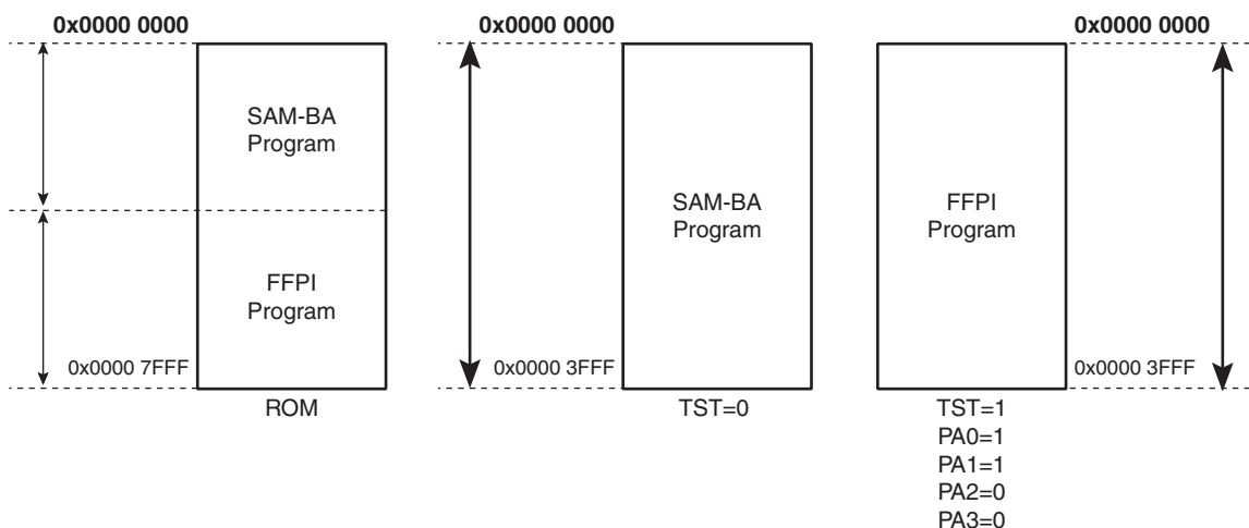
Figure 8-2. ROM Boot Memory Map
