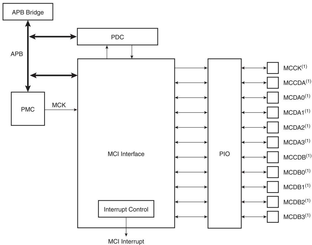
Figure 37-1. Block Diagram
