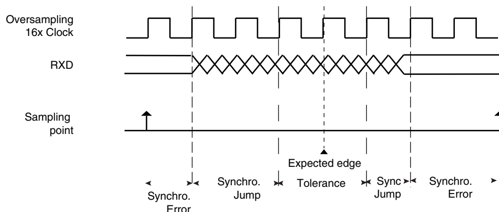
Figure 34-11. Bit Resynchronization
