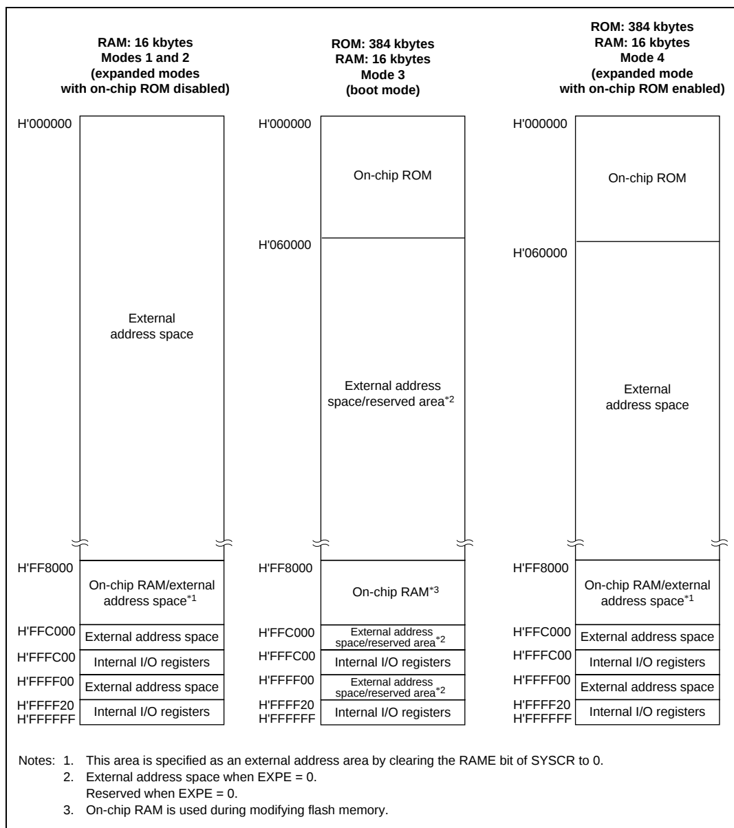
Figure 3.1 Memory Map (1)
