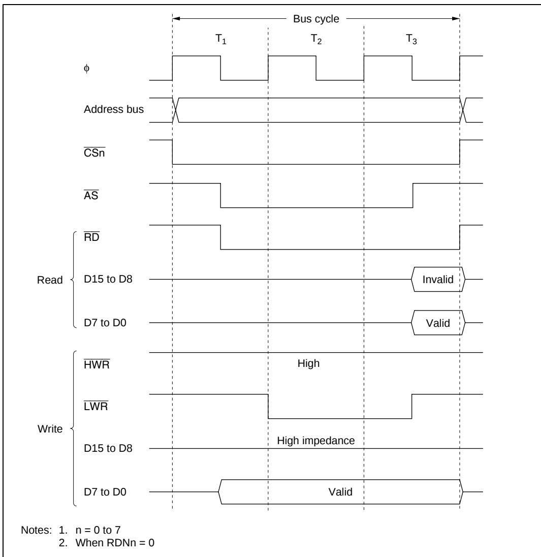
Figure 6.14 Bus Timing for 16-Bit, 3-State Access Space (Odd Address Byte Access)
