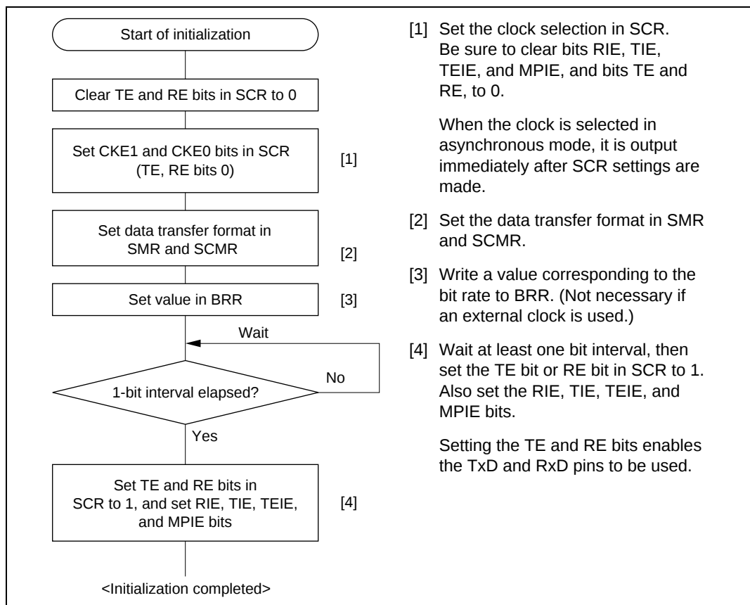
Figure 13.5 Sample SCI Initialization Flowchart
