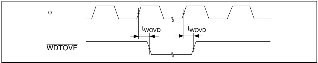
Figure 21.20 WDT Output Timing
