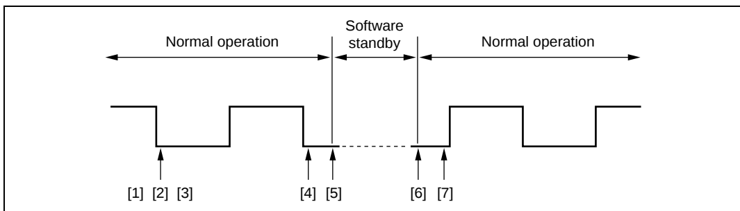
Figure 13.32 Clock Halt and Restart Procedure
