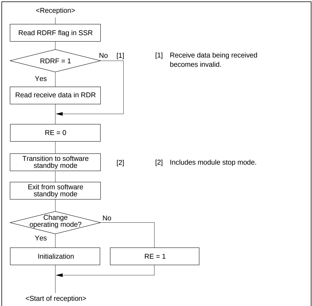
Figure 13.39 Sample Flowchart for Mode Transition during Reception
