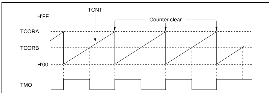
Figure 11.2 Example of Pulse Output
