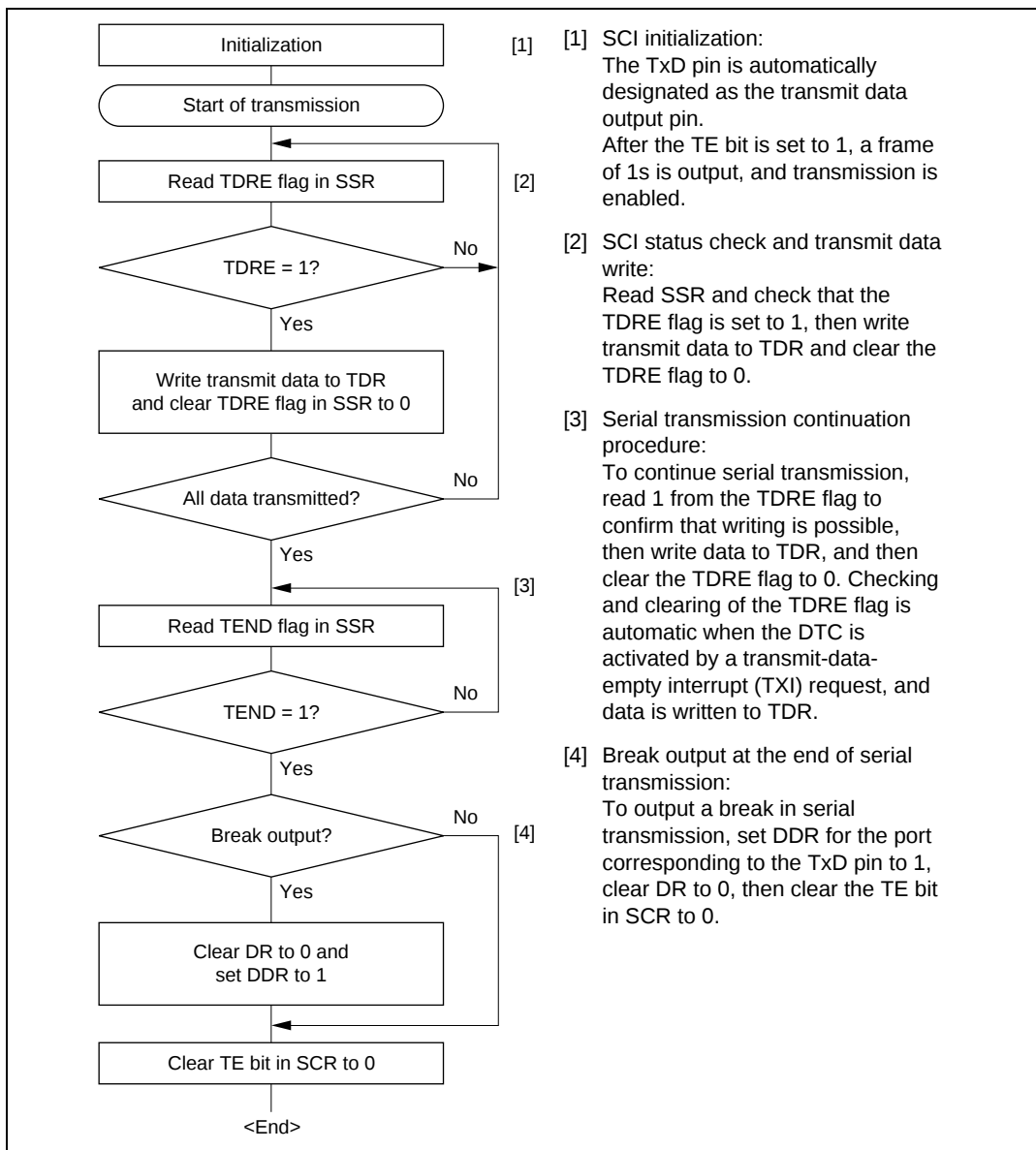
Figure 13.7 Sample Serial Transmission Flowchart
