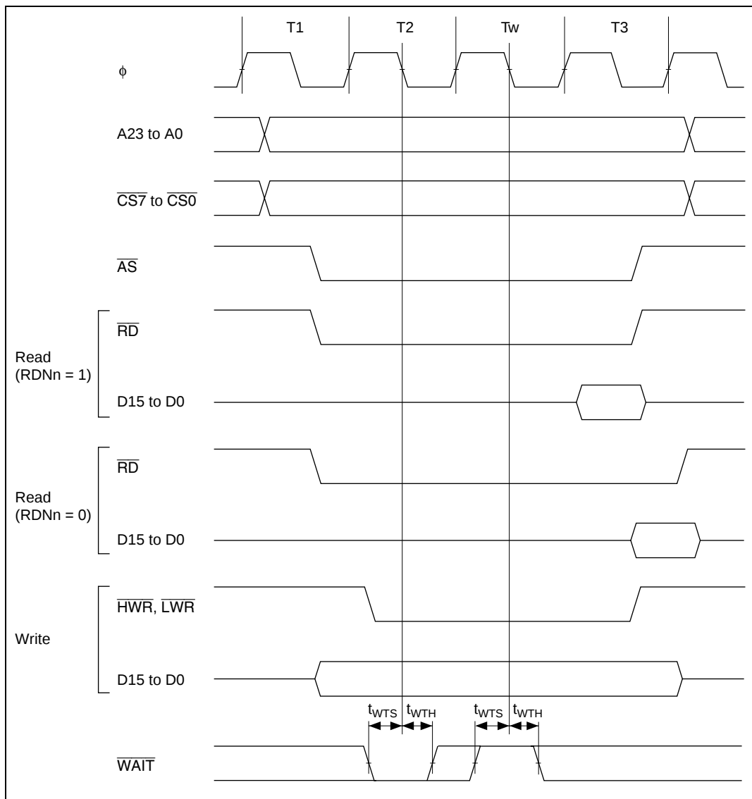
Figure 21.8 Basic Bus Timing: Three-State Access, One Wait
