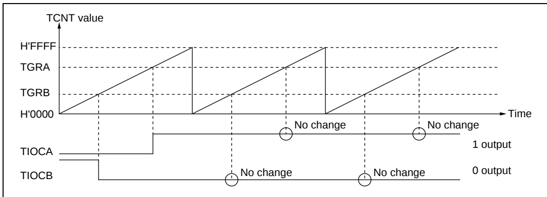
Figure 9.6 Example of 0 Output/1 Output Operation
