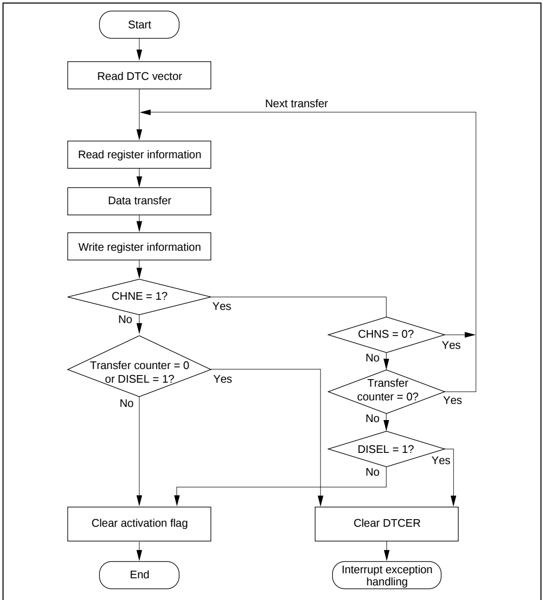
Figure 7.4 Flowchart of DTC Operation
