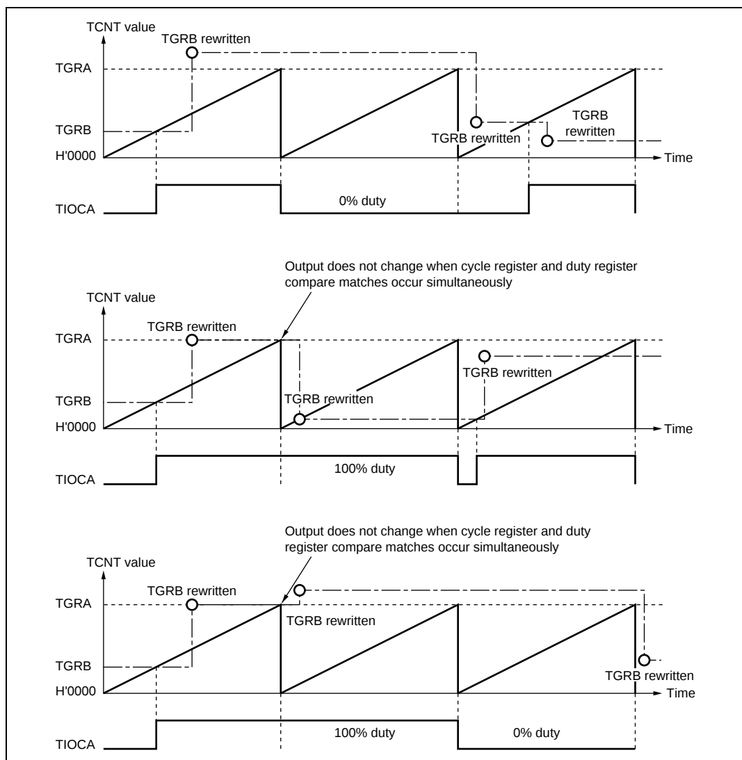
Figure 9.23 Example of PWM Mode Operation (3)
