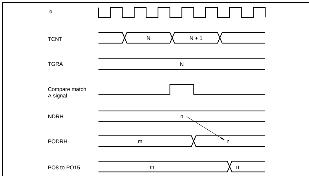
Figure 10.3 Timing of Transfer and Output of NDR Contents (Example)
