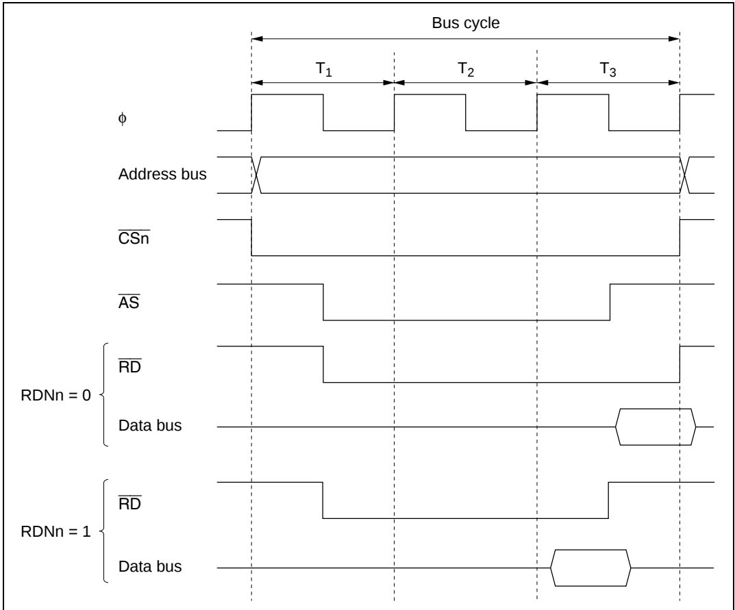
Figure 6.17 Example of Read Strobe Timing
