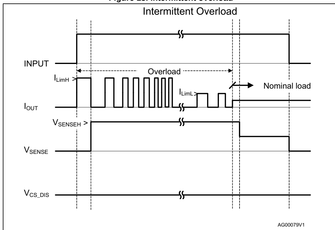
Figure 13. Intermittent overload
