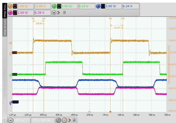
Figure 8-15. Typical TXD, RXD, CANH and CANL Waveforms at 2 Mbps
