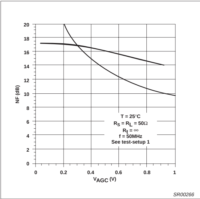
Figure 30. Noise Figure vs V_{\text{AGC}}
