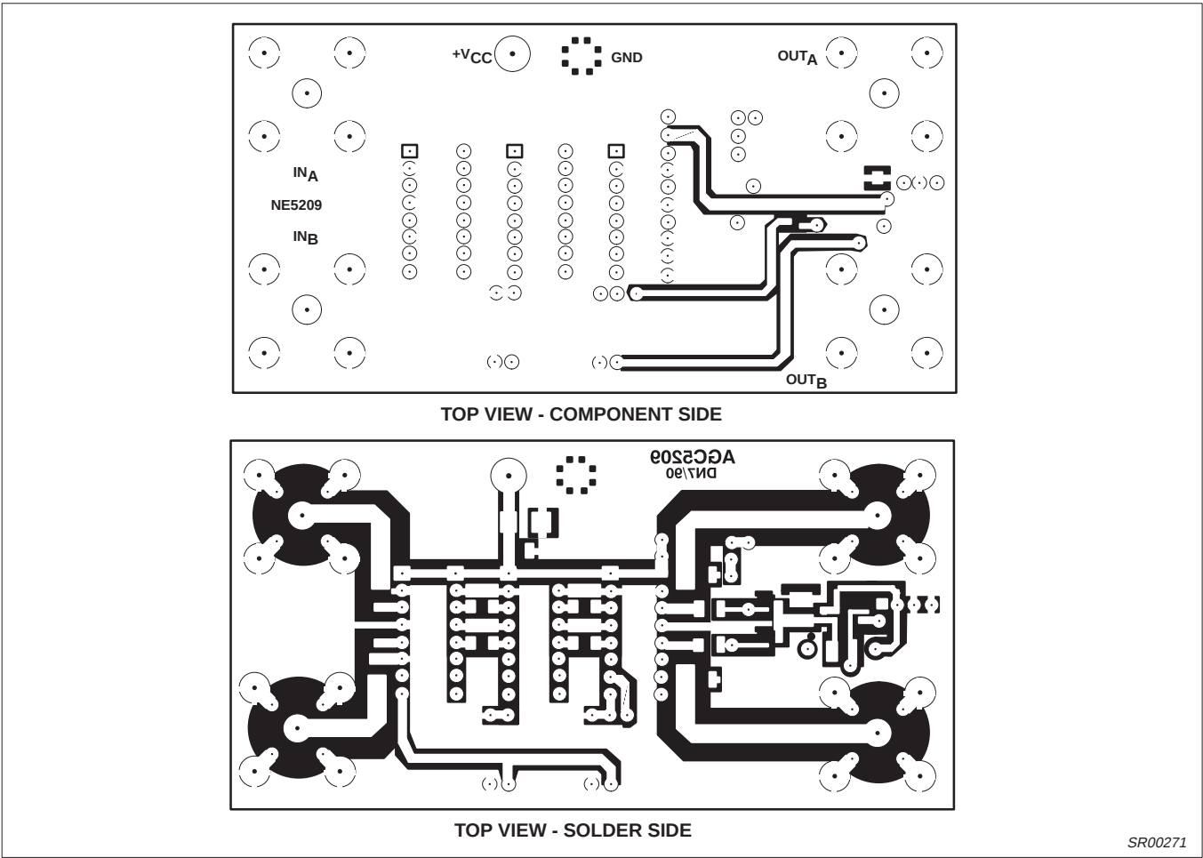
Figure 35. AGC Configuration Using Cascaded SA5209s - Layout
