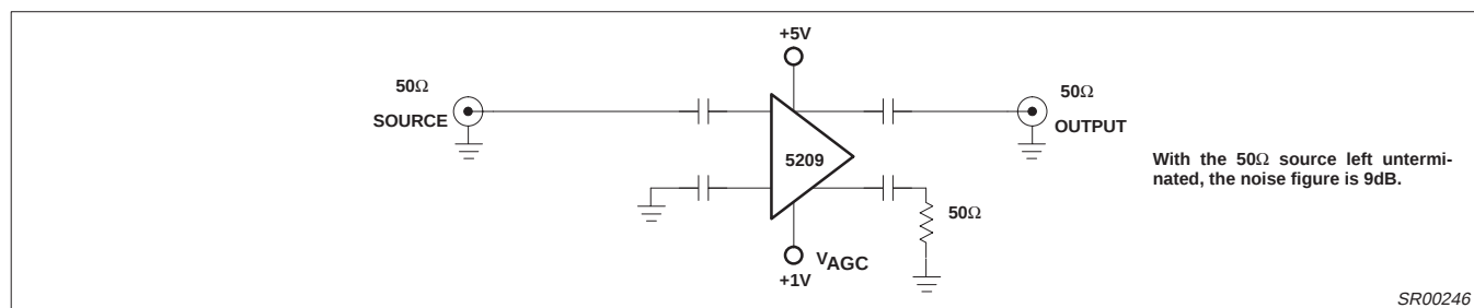
Figure 10. Underterminated Configuration
