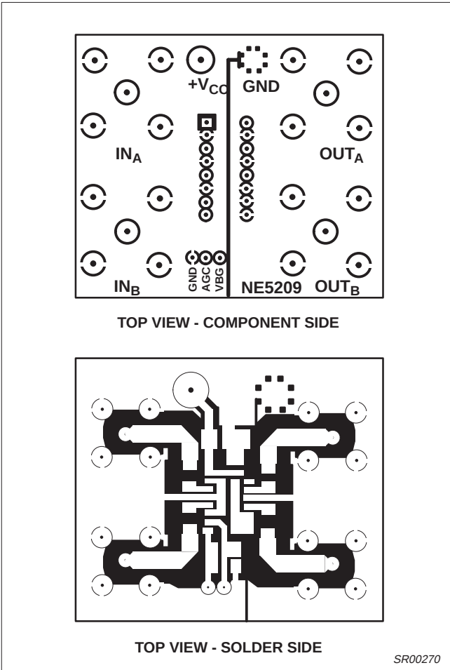
Figure 34. VGA AC Evaluation Board Layout
