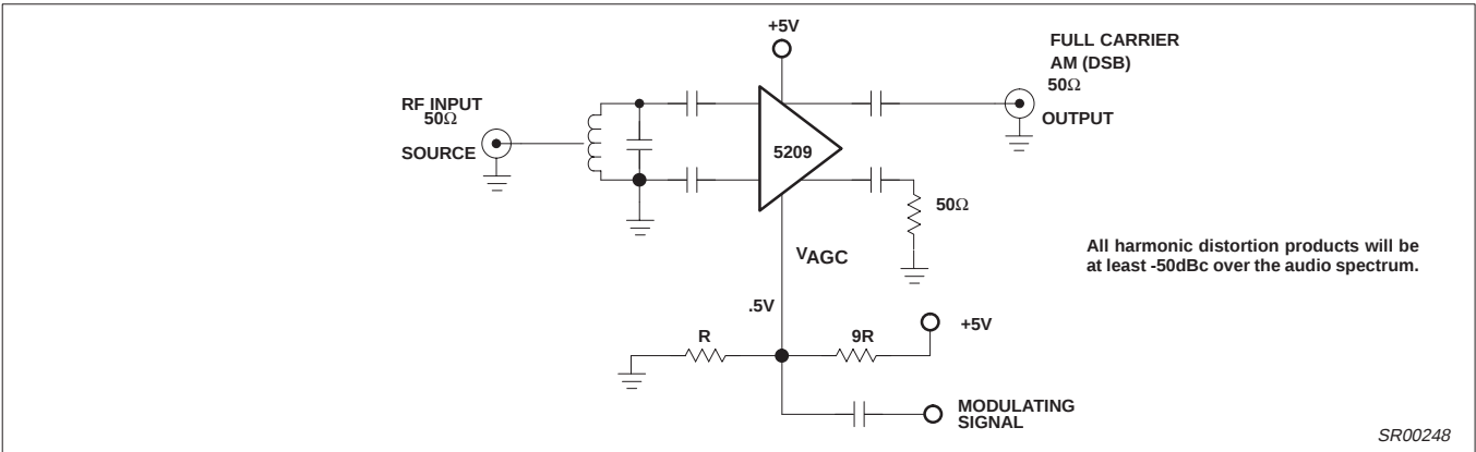
Figure 12. AM Modulator
