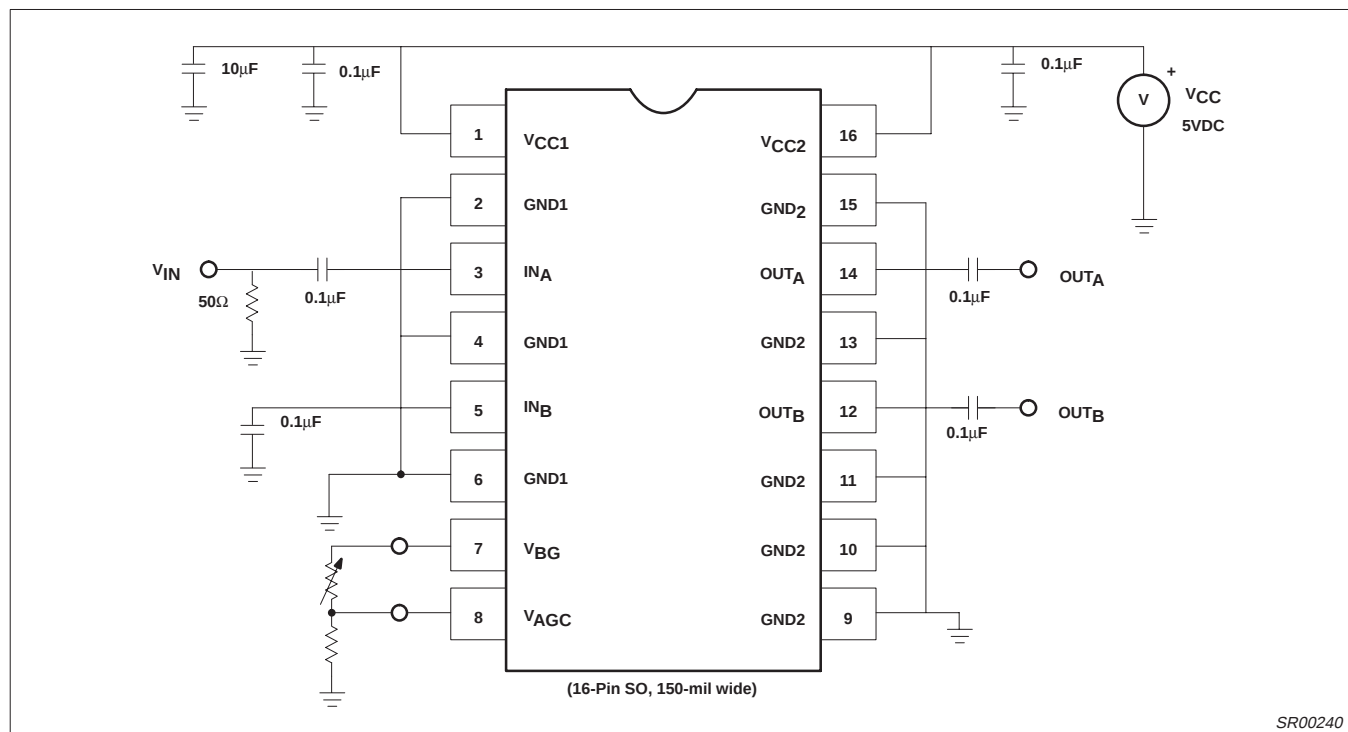
Figure 4. VGA AC Evaluation Board
