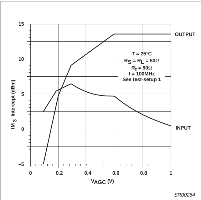
Figure 29. Third-Order Intermodulation Intercept vs V_{\text{AGC}}
