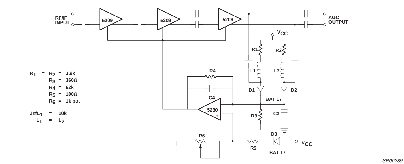
Figure 3. AGC Configuration Using Cascaded SA5209s
