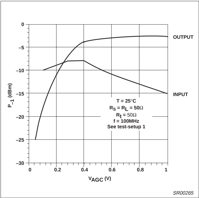
Figure 28. 1dB Gain Compression vs V_{\text{AGC}}
