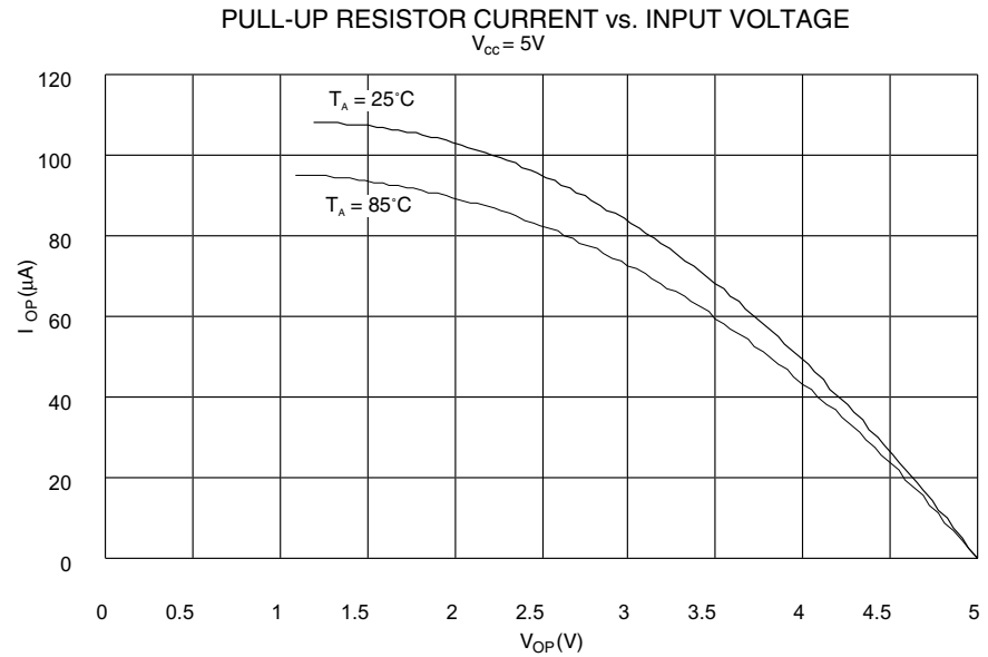
Figure 68. Pull-up Resistor Current vs. Input Voltage
