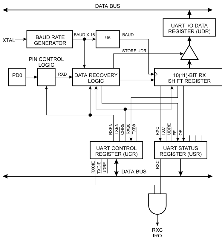
Figure 35. UART Receiver
