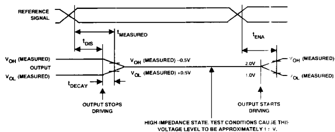
Figure 30. Output Enable/Disable
