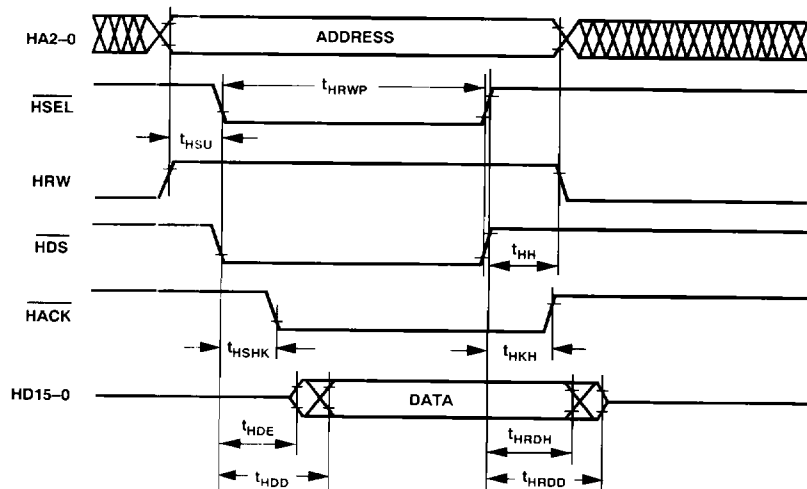
Figure 22. Host Interface Port (HMD1 = 0, HMD0 = 1)
