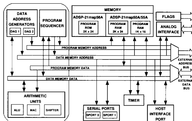
ADSP-2100 BASE ARCHITECTURE
