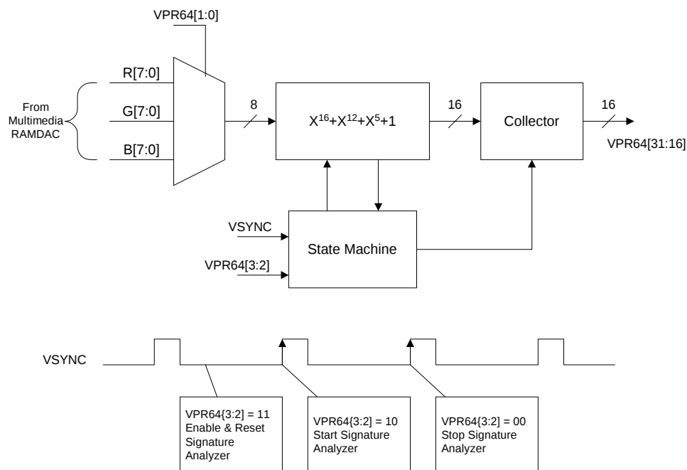
Figure 27: Signature Analyzer Block Diagram
