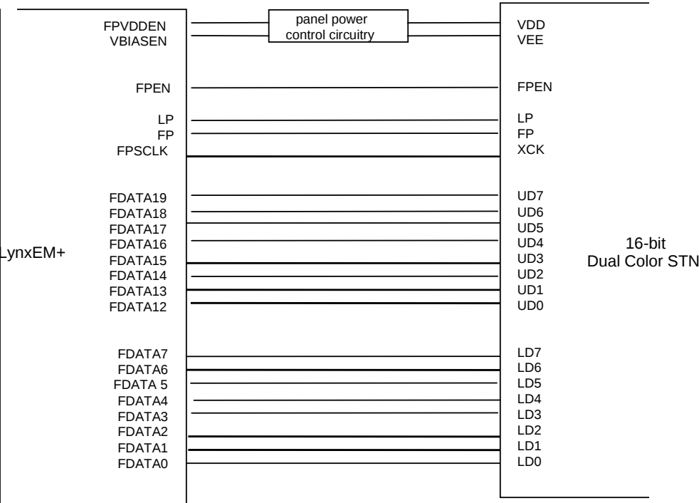
Figure 14: 16-bit DSTN Interface Configuration
