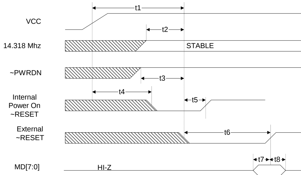
Figure 29: Power-on Reset and Reset Configuration Timing
