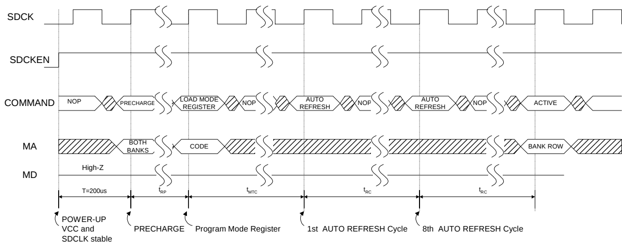
Figure 4: External SGRAM Power-Up and Initialization Sequence
