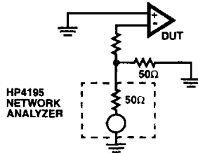
FIGURE 1. TEST CIRCUIT FOR TRANSIMPEDANCE MEASUREMENTS
