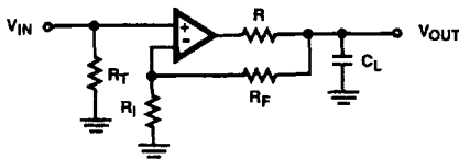
FIGURE 6. PLACEMENT OF THE OUTPUT ISOLATION RESISTOR, R
