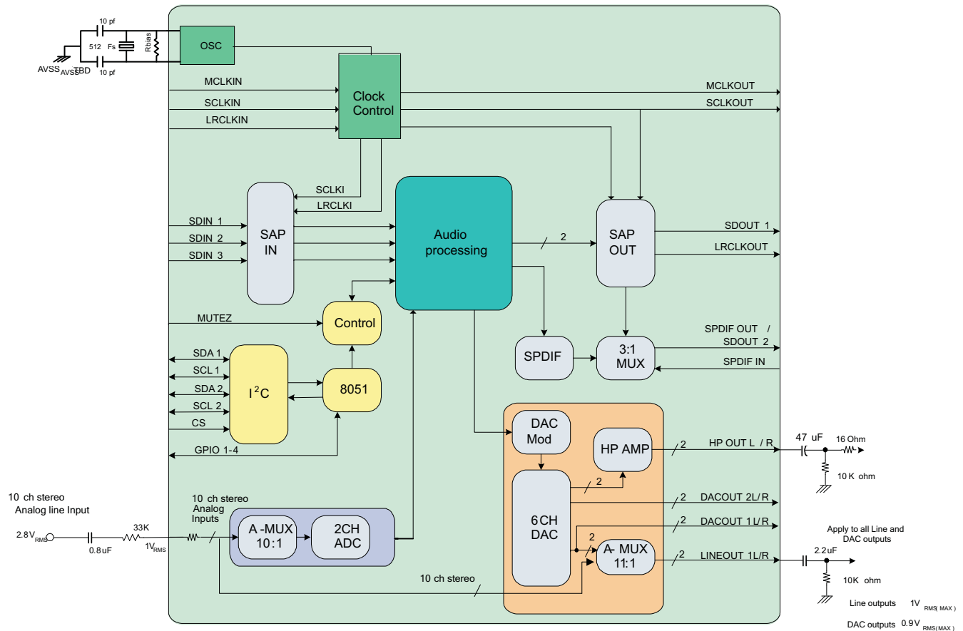
Figure 1. Block Diagram
