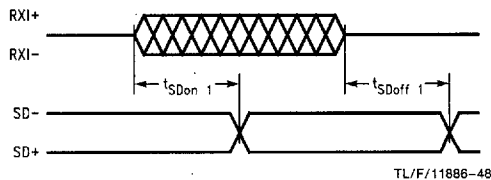
FIGURE 32. Signal Detect Timing (Binary RXI to SD)
