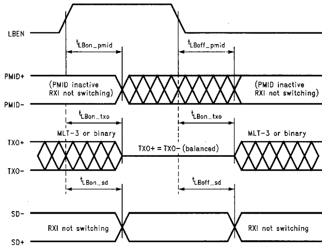
FIGURE 29. Loopback Timing
