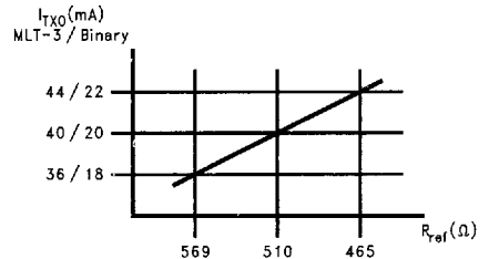
FIGURE 24b. Typical TXO Current vs R_{REF}
