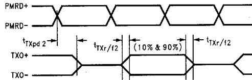
FIGURE 26. TXO Timing (MLT-3)
