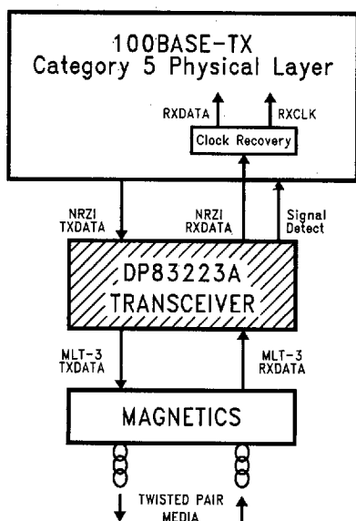
FIGURE 21. Typical 100BASE-TX System Connection
