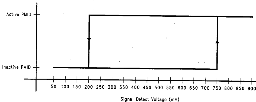
FIGURE 17. Signal Detect
