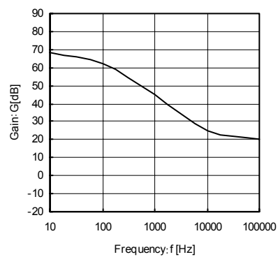
Fig.19 ERRAMP Frequency
