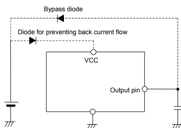
Fig. 39 Bypass diode
