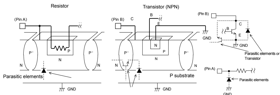
Fig. 40 Example of Simple Bipolar IC Architecture
