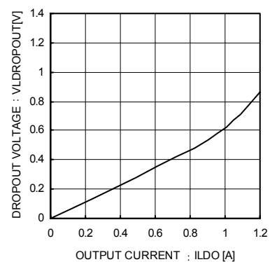
Fig.12 LDO I/O Voltage Differential
