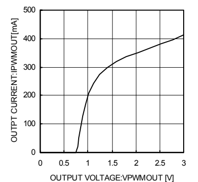
Fig.21 PWM Output Current
