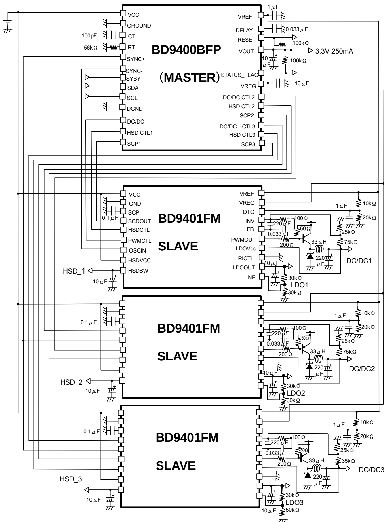
Fig.29 Application Example
