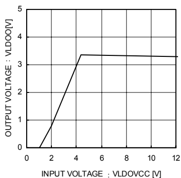
Fig.10 LDO Input Stability (2) (When Vout setting = 3.3 V; Io = 200 mA)
