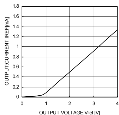
Fig.3 VREF Total Supply Current (BD9401FM)
