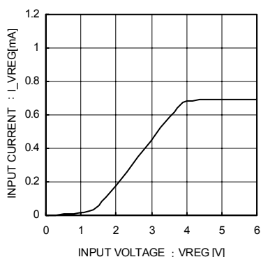
Fig.8 VREG Total Supply Current (BD9403FV)
