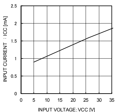
Fig.1 VCC Total Supply Current (BD9401FM)
