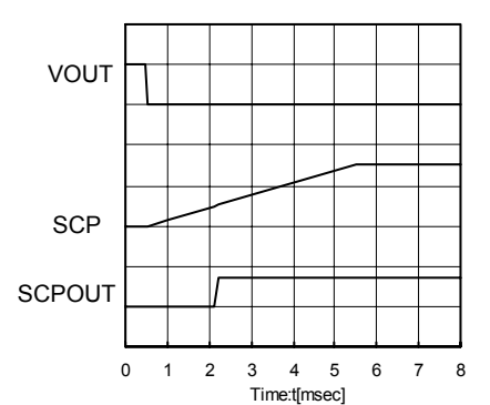
Fig.24 Short Protection Timer
