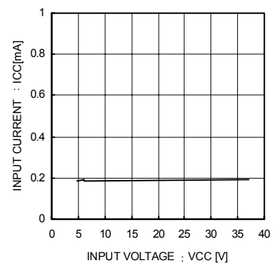
Fig.6 VCC Total Supply Current (BD9403FV)
