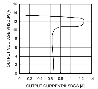
Fig.18 High-Side Switch Load Current
