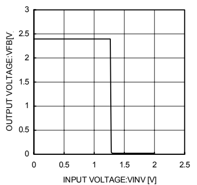
Fig.20 Error Amp I/O (V INV vs V FBI )
