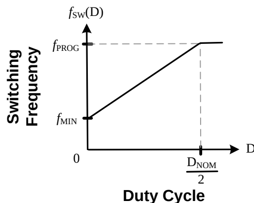
Figure 16. Adaptive Frequency
