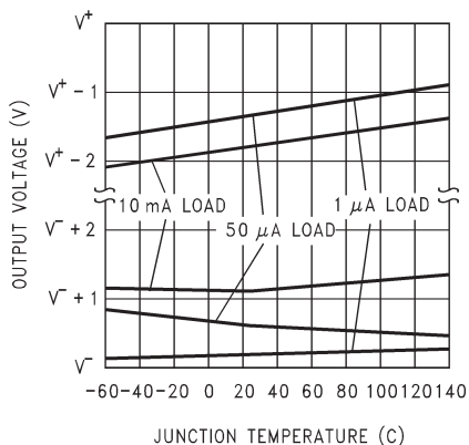
Output Voltage Swing vs Temp. and Current
