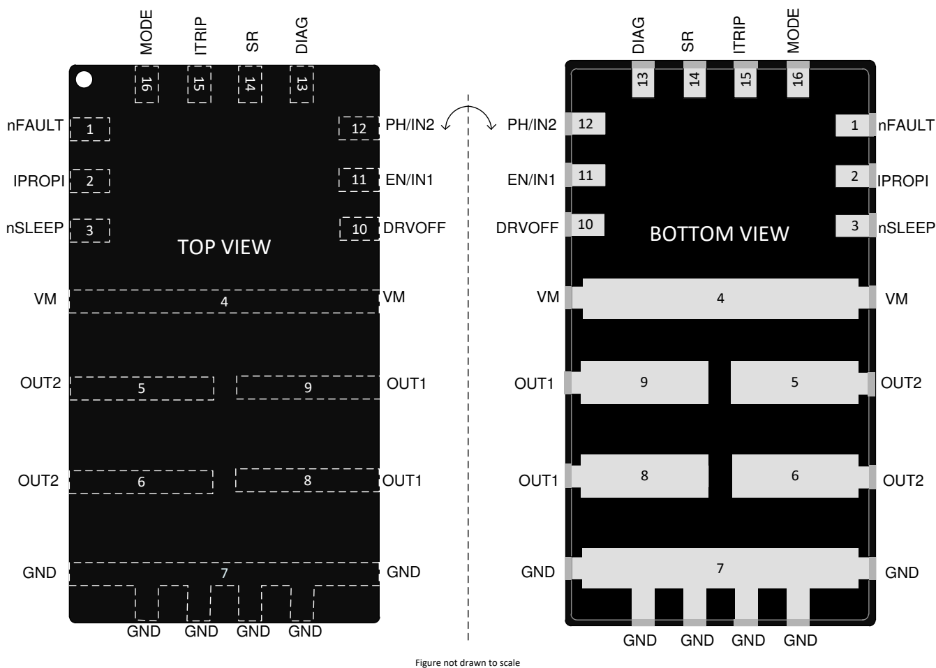
Figure 6-2. DRV8244H-Q1 HW variant in VQFN-HR(16) package
