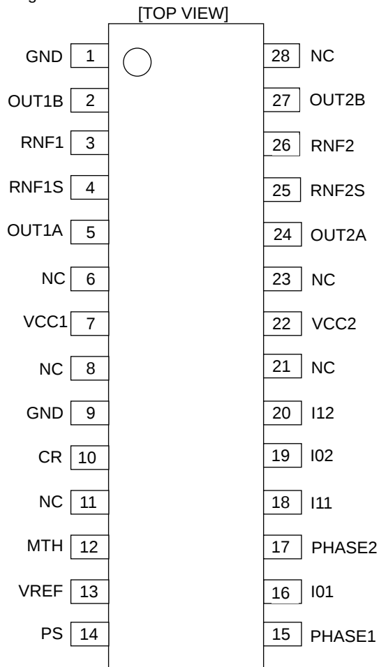
Figure.2 Pin configuration
