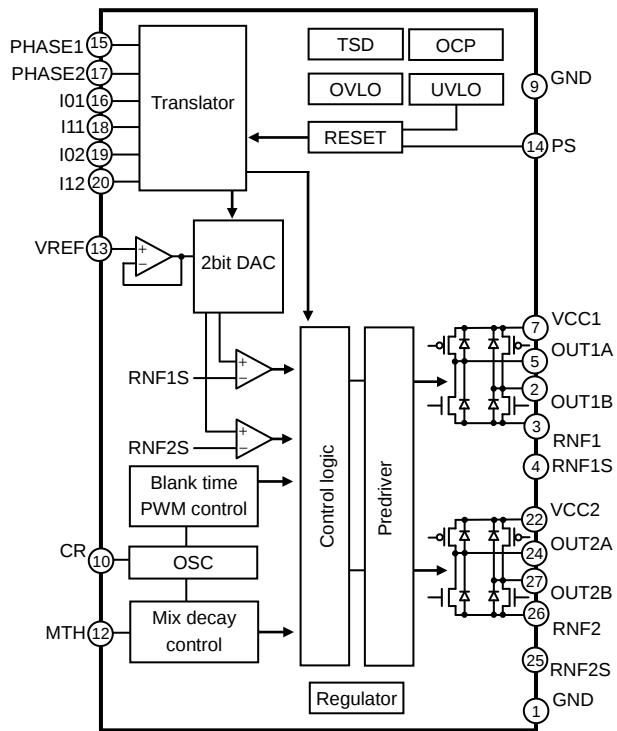
Figure.3 Block Diagram
