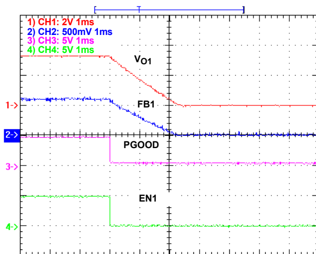
FIGURE 10. ENABLE CONTROL, EN1 = LOW , V_{IN} = 12V , V_{O1} = 3.3V , I_{O1} = 5A
