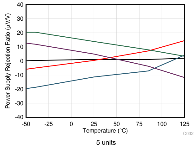
Figure 6-20. PSRR vs Temperature
