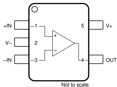
Figure 5-2. OPA391: DCK Package, 5-Pin SC-70 (Top View)
