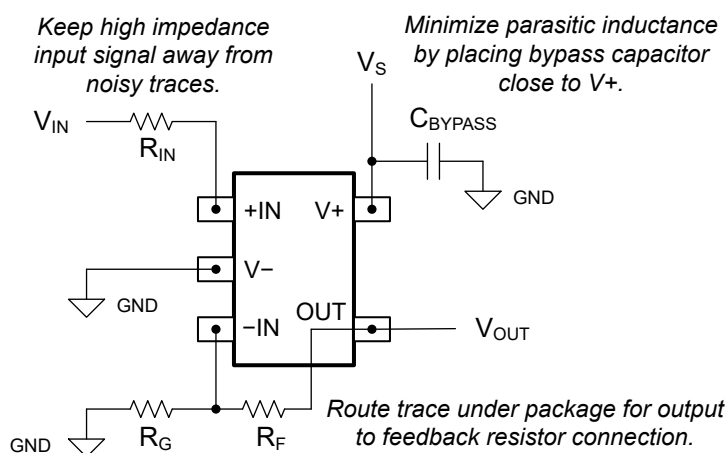
Figure 8-7. Layout Example
