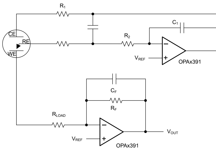
Figure 8-1. Three-Terminal CO Gas Sensor
