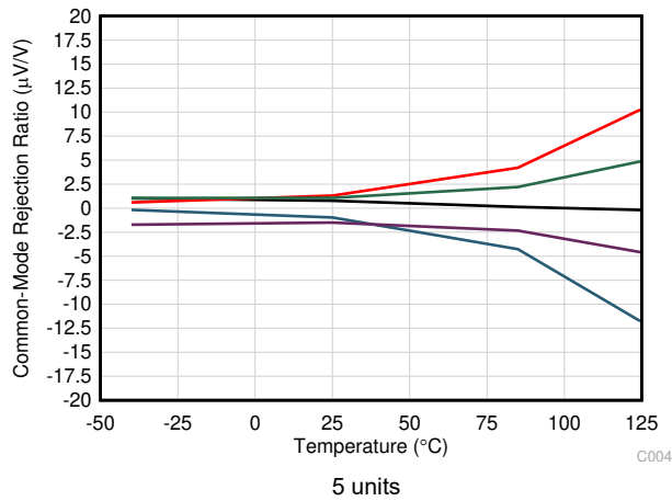
Figure 6-19. CMRR vs Temperature
