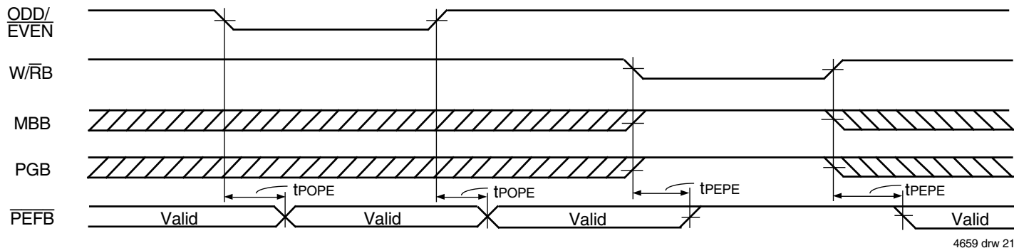
Figure 18. ODD/ \overline{\text{EVEN}} \overline{\text{W/RB}} , MBB, and PGB to \overline{\text{PEFB}} Timing
